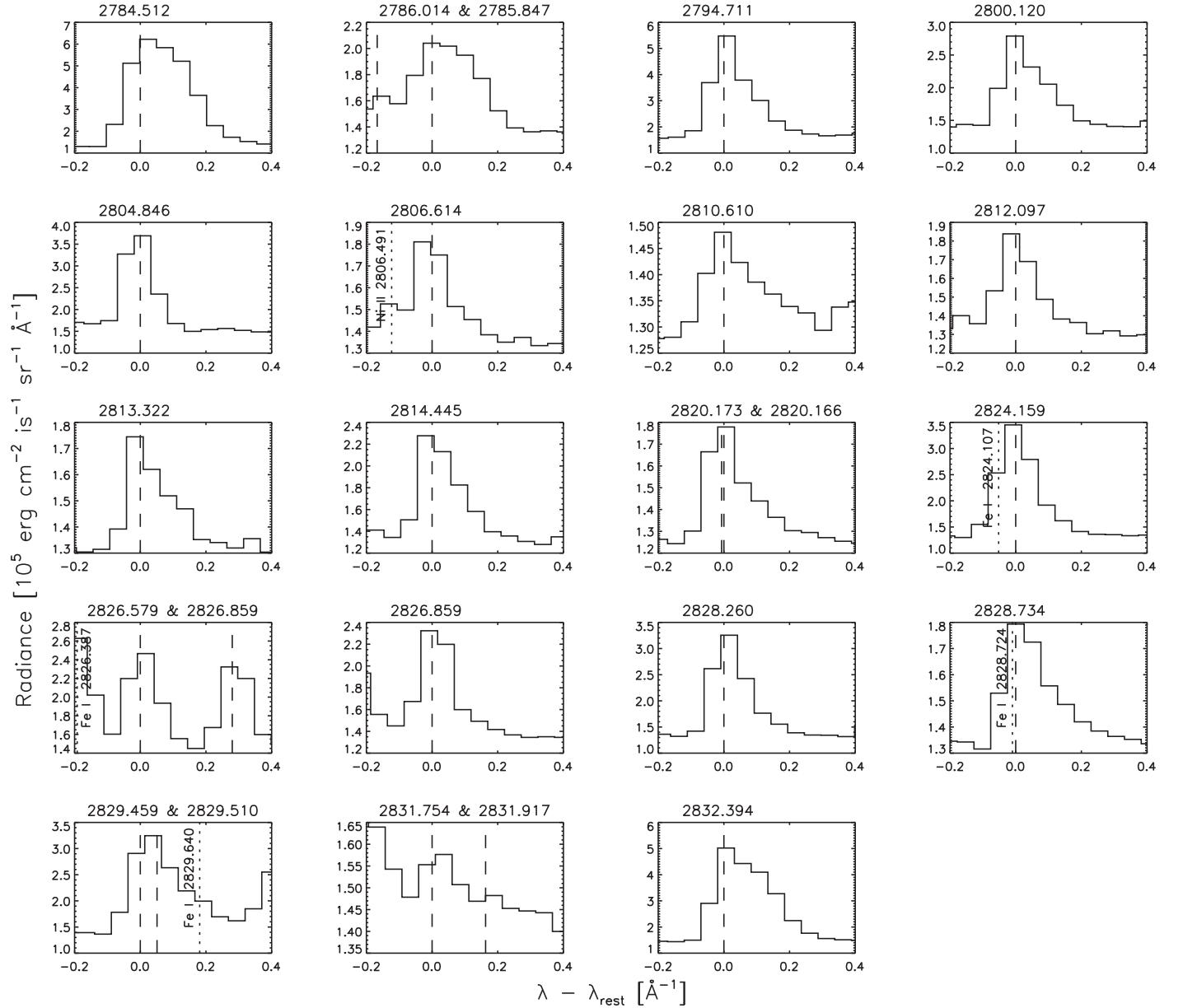
Figure 9. Line profiles in the NUV spectrum of UFB-3 for all definitively identified Fe II lines. All wavelength scales are from -0.2 to 0.4 Å from the rest wavelength, where the stronger Fe II line is used when two are present. Rest wavelengths of Fe II lines and other blends are indicated by dashed and dotted lines, respectively. Many of the Fe II profiles exhibit a red-wing asymmetry with more spectral bins with an intensity greater than or equal to the line half-maximum on the red side than on the blue side.
