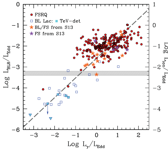
Figure 1. Broad line region luminosity as a function of \gamma -ray luminosity, both normalized to the Eddington luminosity. Different symbols correspond to different classifications, as labelled. The dashed line is the result of a least square fit. The grey stripe indicates the luminosity divide between FSRQs and BL Lacs, located at L_{\text{BLR}}/L_{\text{Edd}} \sim 5 \times 10^{-4} .
