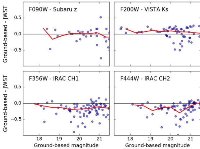
Figure 6. Comparison between NIRC am total magnitudes and catalogs obtained running SE TRACTOR on archival data, at four wavelengths sampled by similar filters by the JWST and the corresponding instrument (with a color correction applied on the basis of theoretical SEDs). The red lines are the medians of the distributions. The overall consistency is good and the typical average offsets are below 0.1–0.2 mag.
