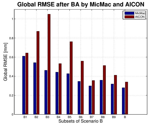
Figure 6: RMSE measured for subsets of Scenario B (described in Table 2), sorted by increasing number of images.
