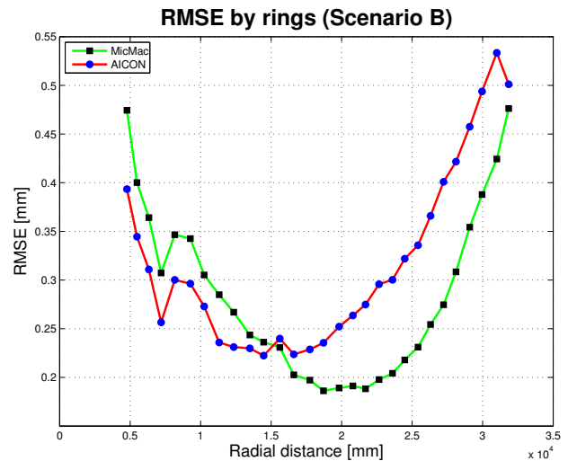
Figure 7: RMSE computed for each ring of targets, identified by their radial distance, for Scenario B.
