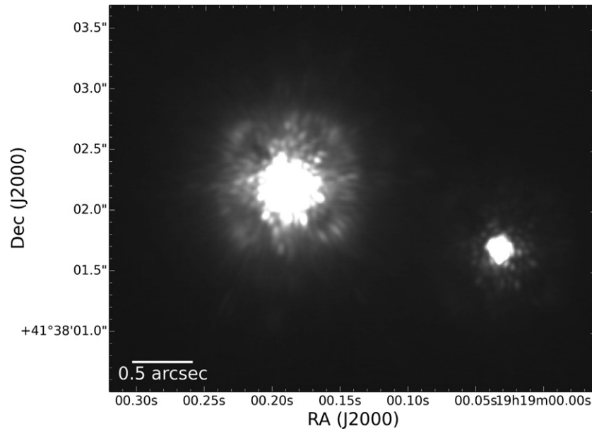
Figure 3. NIRC2 adaptive optics image of Kepler-444. The image was obtained using the K' filter ( 2.124\ \mu\text{m} ) for a total of 378 s of integration time. Declination and right ascension coordinates (J2000.0) are given along the vertical and horizontal axes, respectively.
