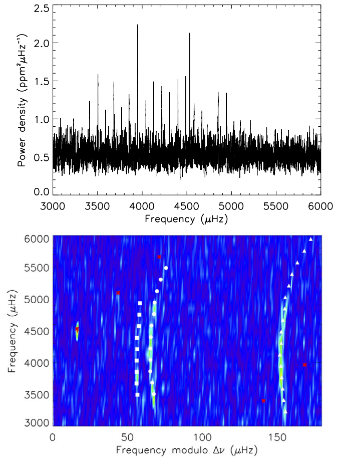
Figure 7. Top panel: frequency–power spectrum of the flux time series of Kepler-444 over the frequency range occupied by the solar-like oscillations. A boxcar filter of width 1.5 \mu\text{Hz} has been applied to enhance p -mode visibility. Bottom panel: power spectrum of the Kepler light curve in échelle format. This is the graphical equivalent to slicing the spectrum into segments of length \Delta\nu = 179.64 \mu\text{Hz} and stacking them one on top of the other. Note that, in order to center the power ridges on the diagram, frequencies have been shifted sideways by subtracting a fixed reference of 25.5 \mu\text{Hz} (i.e., 2000 \mu\text{Hz} \bmod \Delta\nu ). White symbols represent the observed oscillation frequencies. Symbol shapes indicate mode degree: l = 0 (circles), l = 1 (triangles), and l = 2 (squares). Red asterisks mark the harmonics of the inverse of the Kepler long-cadence period ( \Delta t \sim 30 minutes), not all of which are present in these data. These artifacts appear in the power spectra of Kepler short-cadence time series.
