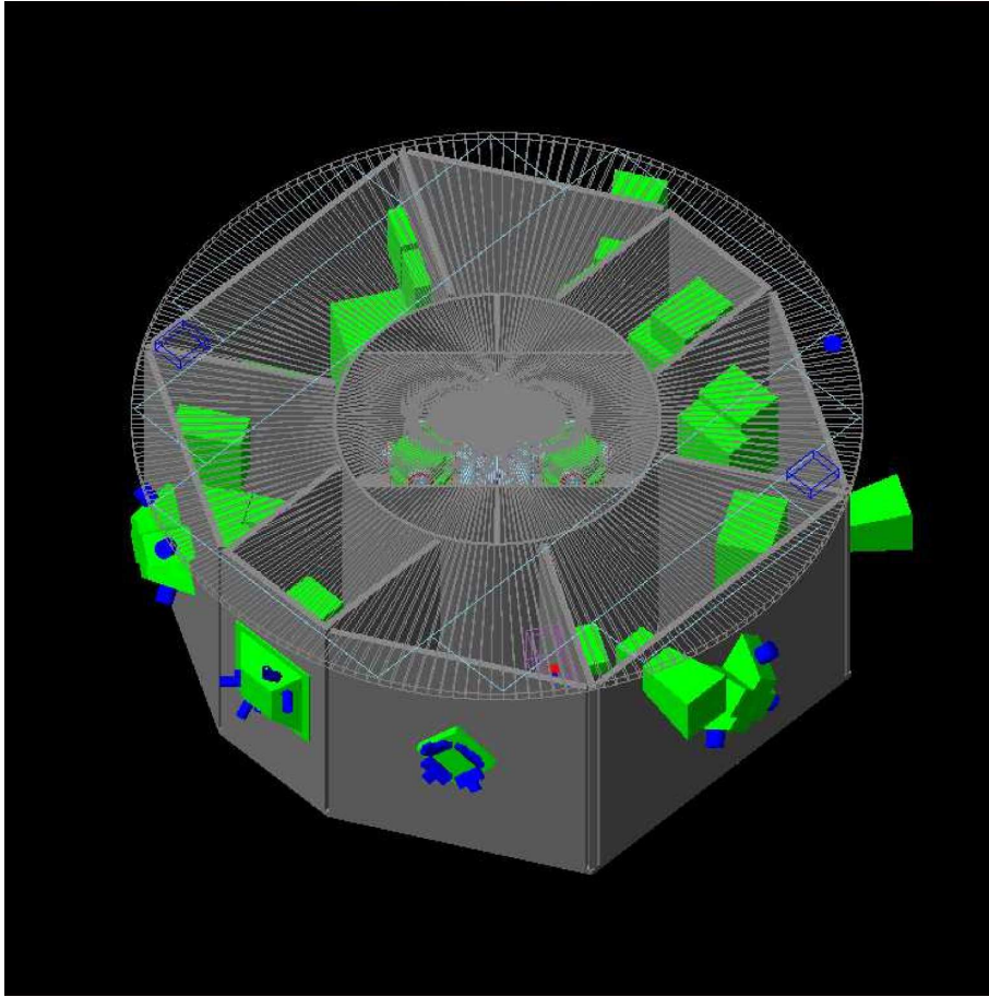
Figure 4. Sketch of the LISA-PF geometry.
