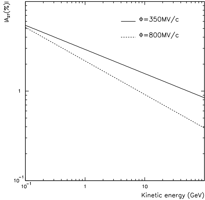
Figure 2. Parameterizations of 27-day GCR intensity fractional variations in 2015. Variations must be intended both positive and negative with respect to the average overall GCR observed intensity. Solid ( \phi=350 MV/c) and dashed ( \phi=800 MV/c) lines represent the maximum and minimum expected values, respectively.
