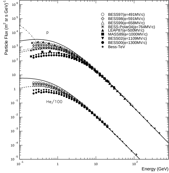
Figure 1. Estimated GCR proton and helium nucleus energy spectra during the second half of 2015. Maximum (solid lines) and minimum (dashed lines) projections are reported. Helium data are scaled by a factor of 100 in order not to superpose data and lines. The dot-dashed curves represent the proton flux observed by the PAMELA experiment during the Forbush decrease of December 14th 2006 between 1650UT and 2235UT [30]. Galactic (bottom dot-dashed line) and solar (top dot-dashed line) proton components appear separated.
