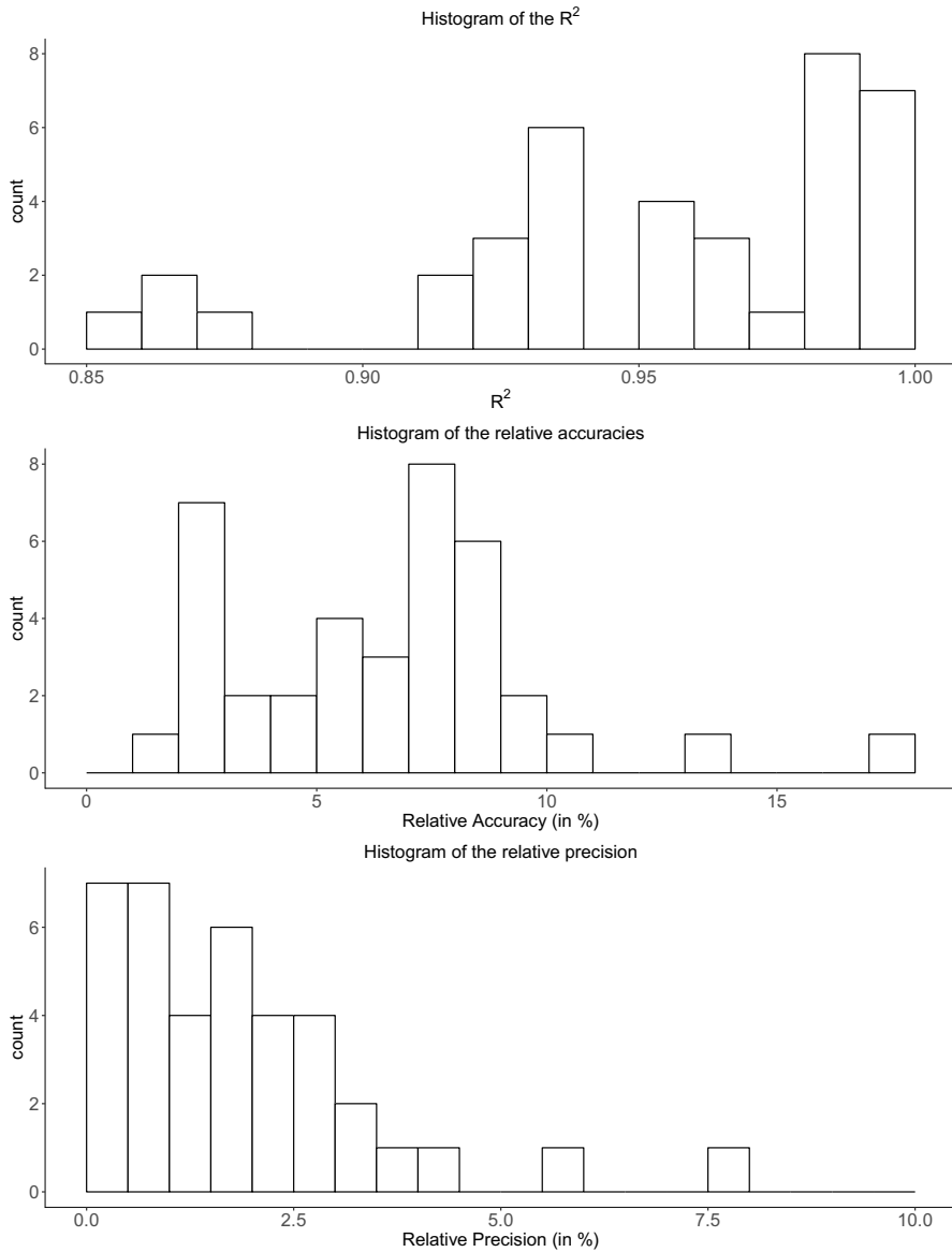
Fig. 6 Histogram showing the adj- R^2 (top panel), accuracy (central panel), and precision (bottom panel; both in terms of relative differences) of the 38 relations presented in Moya et al. (2018) (Figure credit: Moya et al. 2018)
