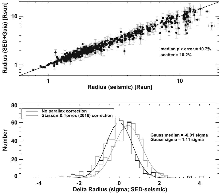
Fig. 4 Comparison of stellar radii obtained from SED+parallax versus stellar radii from asteroseismology. (Top) Direct comparison. (Bottom) Histogram of differences in units of measurement uncertainty; a small offset is explained by the systematic error in the Gaia DR1 parallaxes reported by Stassun and Torres (2016b). Image reproduced with permission from Stassun et al. (2018), copyright by AAS
