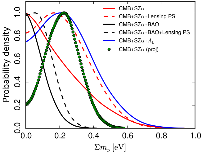
Fig. 12. Constraints on \Sigma m_v from a joint analysis of the cluster counts and primary CMB. The solid and dashed, red and black lines reproduce the marginalized posterior distributions from Fig. 11. The solid blue line is the posterior from a similar analysis, but marginalized over the additional parameter A_L (see text). If applied to the present Planck cluster cosmology sample, a future mass calibration of 1 - b = 0.78 \pm 0.01 would result in the bold, dotted green posterior curve.
