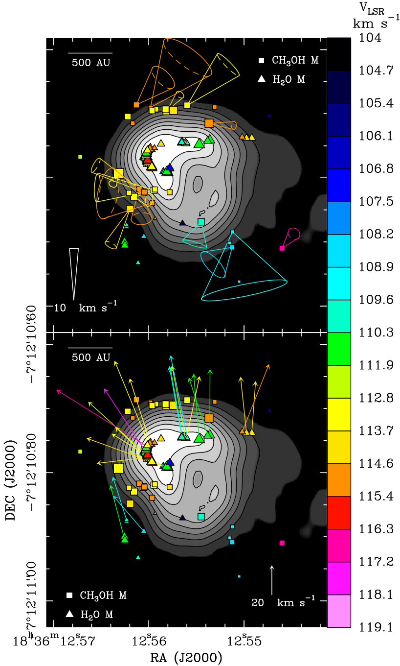
Fig. 10. Three-dimensional motions of the methanol (upper panel) and water (lower panel) masers in G24.78+0.08 A1N. In both panels, the gray-scale image and black contours (10–90%, at step of 10% of the image peak of 11 \text{ mJy beam}^{-1} ) reproduce the VLA A-Array 7 mm continuum. Colored triangles and squares report the absolute positions (evaluated at the date 2003 September 4) of the 22 GHz water and 6.7 GHz methanol masers, respectively, with colors denoting V_{\text{LSR}} as coded in the wedge on the right of the plot. In the upper panel, the 3D velocities of the methanol masers are shown with cones, with opening angle representing the uncertainty in the direction of motion and base ellipticity proportional to the ratio of the velocity components on the plane of the sky and along the line of sight. The white cone in the left bottom corner of the panel gives the scale for the velocity amplitude. In the lower panel, the sky-plane velocities of the water masers are indicated with arrows. The white arrow at the right bottom shows the velocity scale.
