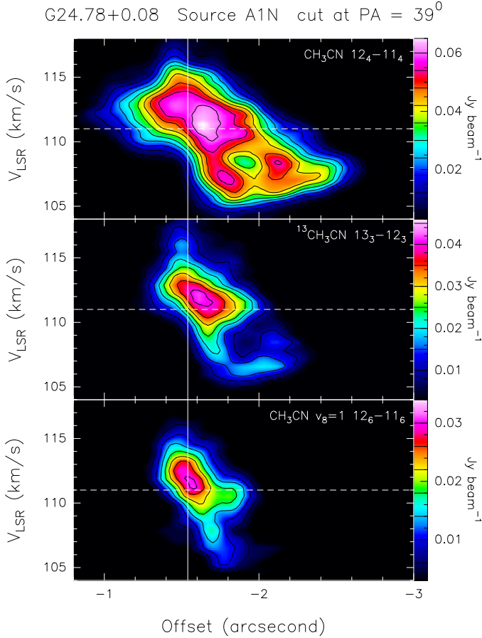
Fig. 12. P-V plots of the \text{CH}_3\text{CN} 12 4 –11 4 , ^{13}\text{CH}_3\text{CN} 13 3 –12 3 and \text{CH}_3\text{CN} v_8=1 12 6 –11 6 lines are presented in the upper, middle and lower panels, respectively. The intensity scale is shown in the wedge on the right of each panel. The cut axis along which positions are evaluated is the major axis of the H30 \alpha outflow (indicated with a black dashed line in Fig. 9). To produce the P-V plots, we have averaged the emission inside a strip extending \pm 0''.3 above and below the cut axis, including only the HII region and its surroundings.
