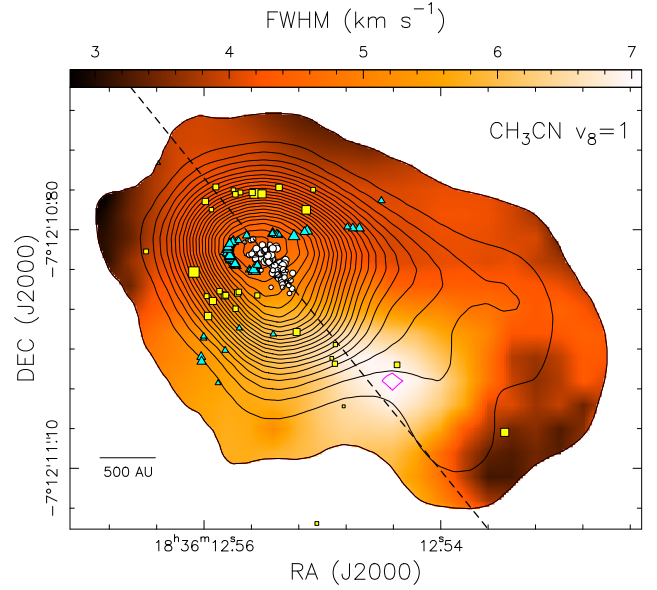
Fig. 13. Color map showing the distribution of line width determined by simultaneously fitting the emission of ten unblended, vibrationally excited transitions of \text{CH}_3\text{CN} with the XCLASS package (see Sect. 3 for details). The field of view corresponds with the area of the HC HII region in G24.78+0.08 A1N. The black contours reproduce the JVLA A-Array 1.3 cm continuum (plotting the same levels as in Fig. 4, upper panel). The magenta contour represents the level of FWHM = 7 \text{ km s}^{-1} , and delimites the local maximum in line width LW-CS. The white dots mark the channel peak positions of the H30 \alpha line emission, and the dashed black line marks the axis of their spatial distribution. The cyan triangles and yellow squares have the same meaning as in Fig. 9.
