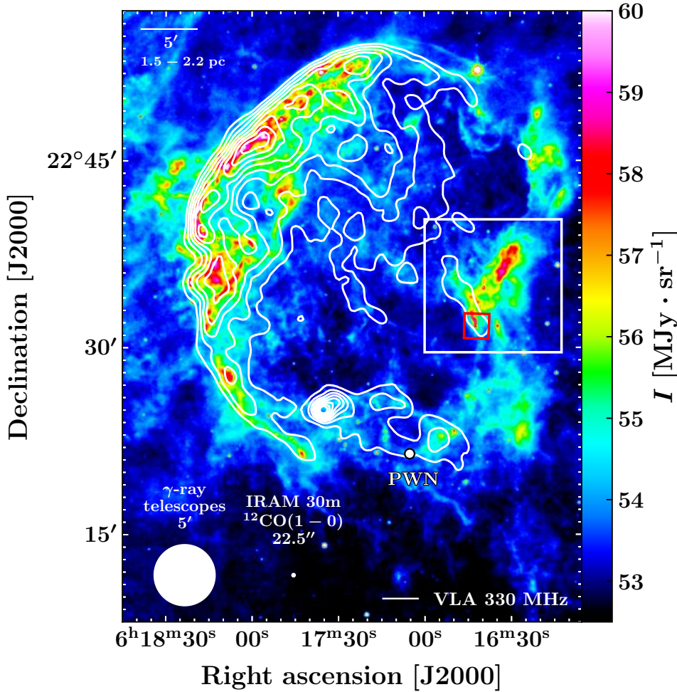
Fig. 1. Spitzer /MIPS map (colors) of IC443 at 24\mu\text{m} (Pinheiro Gonçalves et al. 2011; Noriega-Crespo et al. 2009). In contours, the VLA emission map shows the morphology of the synchrotron emission at 330 MHz (Claussen et al. 1997). The white dot indicates the position of the PWN wind (Olbert et al. 2001b). The red box represents one of the fields observed by Spitzer -IRS (Neufeld et al. 2004), corresponding roughly to the G region defined by Huang et al. (1986). The white box represents the 10' \times 10' field of our observations called “the extended G region”. The IRAM 30 m instrumental beam diameter corresponding to the ^{12}\text{CO}(1-0) transition and the size of the typical PSF of \gamma -ray telescopes ( 5' ) are indicated by white disks in the bottom left corner of the figure.
