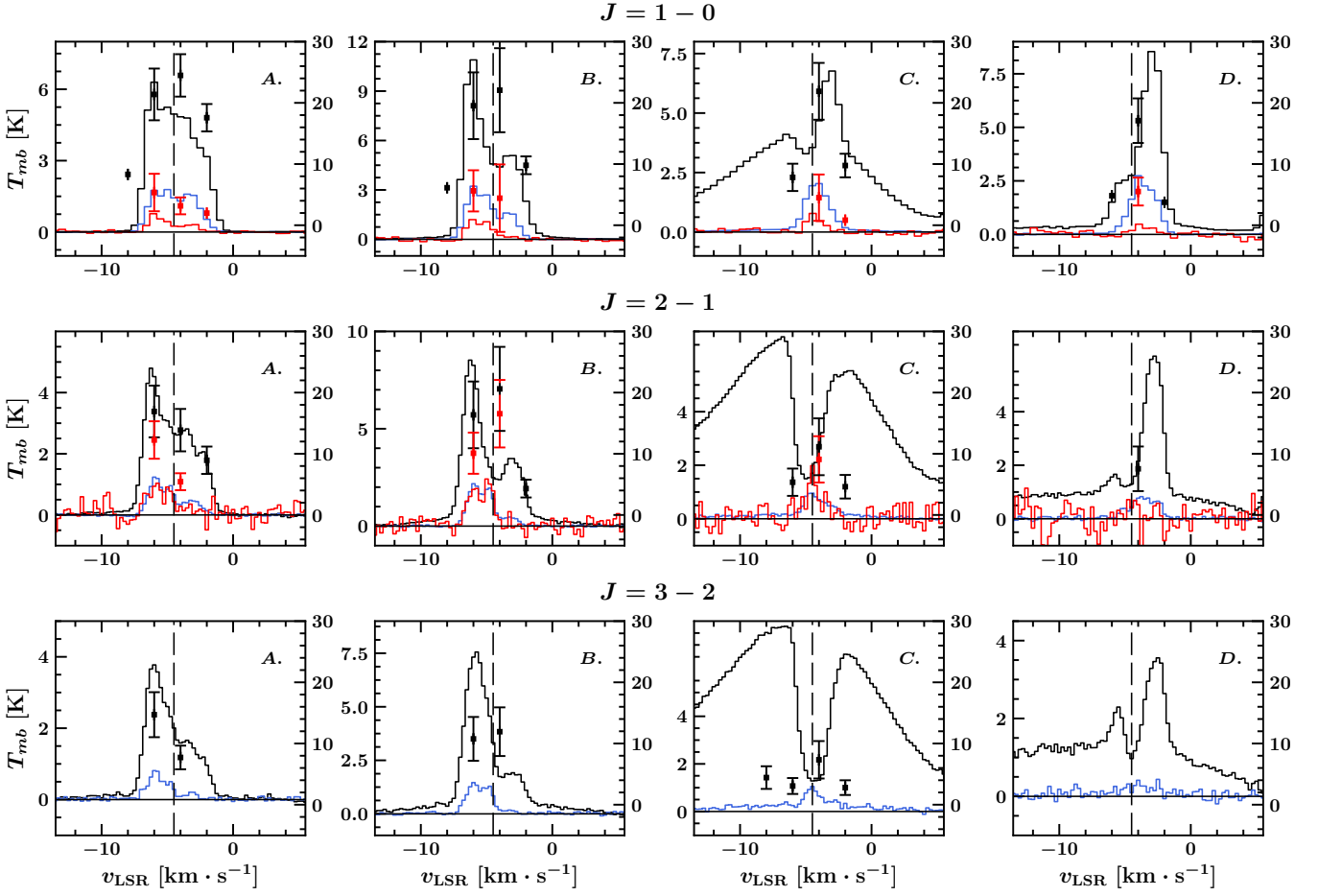
Fig. F.1. Spectra obtained over the region of the four boxes defined in Fig. 6, for the following lines: 12 CO (in black), 13 CO (in blue), and C 18 O (in red). First row: (1–0) transition, second row: (2–1) transition, and third row: (3–2) transition for: A, the cloudlet; B, the ring-like structure; C, the shocked clump; and D, the shocked knot. Spectral cubes were resampled to allow a direct comparison between the different spectra. Spatial resolutions of all transitions were modified to the nominal resolution of C 18 O(2–1), \theta = 30.2'' . Spectral resolution were set to 0.5 km s -1 for the IRAM 30 m data, and 0.25 km s -1 for APEX data. On both panels, the v_{LSR} of IC443 is indicated with a vertical dashed line (at -4.5 km s -1 ). The black data points with error bars represent the measurements of the optical depth \tau corresponding to each channel of these spectra resampled with a spectral resolution of 2 km s -1 , using the [ 12 CO]/[ 13 CO] ratio as a tracer, and the red data points represent the measurements of the optical depth obtained using the [ 12 CO]/[C 18 O] ratio. The adopted values for the isotopic ratios are based on the results of Sect. 4.2.1 and indicated in Table 5.
