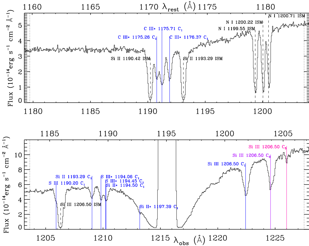
Fig. A.1. 2013 spectrum of NGC 5548. The vertical axis is the flux in units of 10^{-14} \text{ erg s}^{-1} \text{ cm}^{-2} \text{ Å}^{-1} , and the quasar-rest-frame and observer-frame wavelengths are given in Angstroms on the top and bottom of each sub-plot, respectively. Each of the six kinematic components of the outflow shows absorption troughs from several ions. We place a vertical mark at the expected center of each absorption trough (following the velocity template of Si IV and N V) and state the ion, rest-wavelength and component number ( C_1 – C_6 ). We also assign a color to each component number that ranges from blue ( C_1 ) to red ( C_6 ). Absorption lines from the ISM are likewise marked in black with dashed lines.
