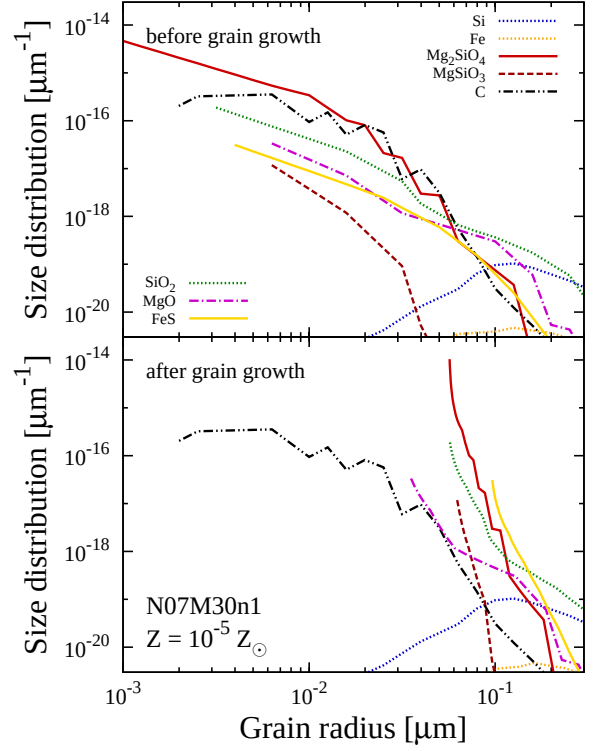
Figure 7. Size distribution function n_i \varphi_i / n_H of dust species i before ( n_H = 0.1 \text{ cm}^{-3} ) and after ( n_H = 10^{16} \text{ cm}^{-3} ) grain growth for our N07M30n1 model with Z = 10^{-5} Z_{\odot} . Size of all species but for C and Si grains increases by accretion of heavy elements. C and Si grains do not grow because the key species, C and Si atoms, are depleted onto CO and SiO molecules, respectively.
