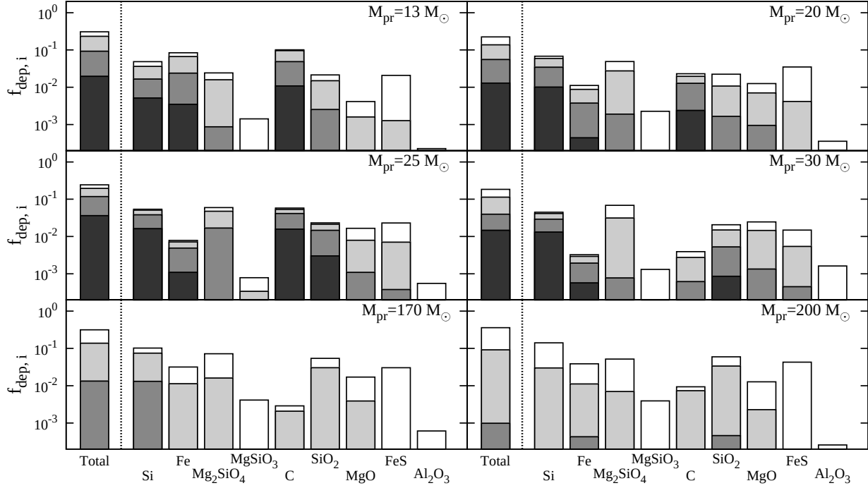
Figure 3. Mass fraction f_{\text{dep},i} of grain species i relative to the total metal mass for supernova model of N07. Each histogram represents the mass fraction for n0, n0.1, n1, and n10 model from top to bottom. The first histogram represents the depletion factor f_{\text{dep}} whereas the other histograms show the contribution of each dust species.
