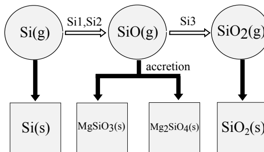
Figure 1. Chemical network of silicon (white arrows) which are included in our one-zone calculations. We also consider accretion of gas-phase species onto grains (indicated by black arrows). The reaction tabs above the arrows are identical with the reaction numbers in Table 1. Circles and squares depict gas-phase (g) and solid-phase (s) species, respectively.
