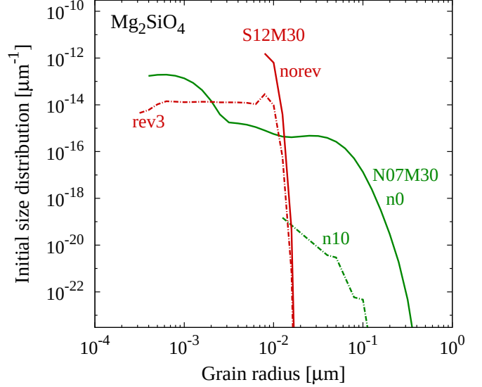
Figure 5. Initial size distribution of Mg 2 SiO 4 grains for the N07 (green) and S12 (red) models without the effect of dust destruction (solid) and with the largest efficiency of dust destruction among their reverse shock models (dot-dashed).
