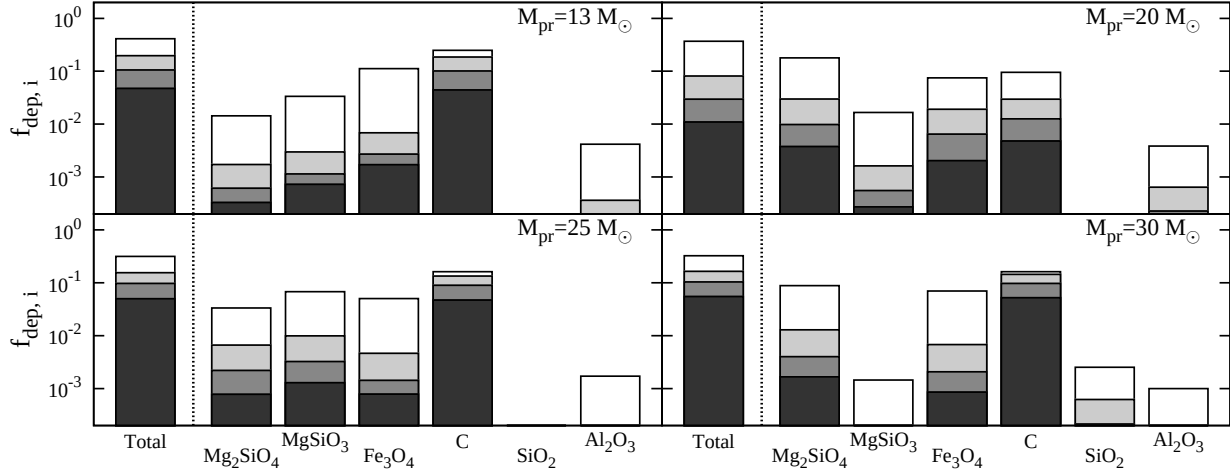
Figure 4. Same as Figure 3 but for models by S12.
