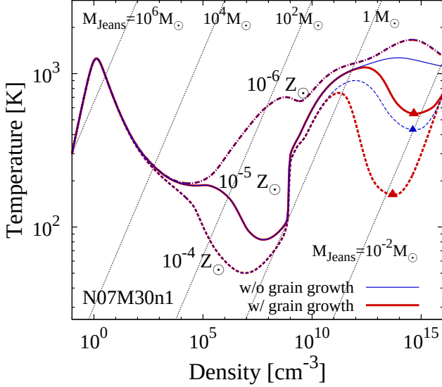
Figure 6. Temperature evolution as a function of the hydrogen number density of the cloud centers for our N07M30n1 model with metallicities Z = 10^{-6} Z_{\odot} (dot-dashed), 10^{-5} Z_{\odot} (solid), and 10^{-4} Z_{\odot} (dashed), respectively. Red thick and blue thin curves depict the cases with and without grain growth, respectively. Triangles are plotted at the states where the fragmentation condition (see text) is met.
