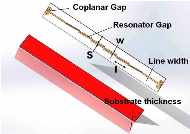
Fig. 4. Typical bandpass filter on alumina substrate showing the microstrip coupled lines and the nomenclature of the lines length (l), width (w), and gap (s). The filter backside (ground plane) is metalized (Au 2 \mu\text{m} ). Parameter values are given in Table III.
