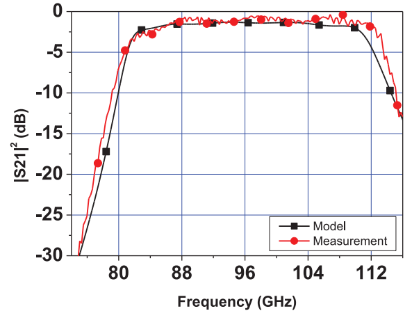
Fig. 13. Graph of the 85–109-GHz bandpass filter transmission with the measured (red circles) and modelled (black squares) responses.
