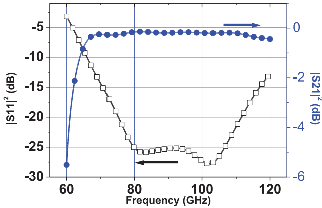
Fig. 15. Simulated reflection (left scale) and transmission (right scale) coefficients of the WR10 waveguide-to-microstrip line transition of Fig. 4 (parameters given in Table IV).
