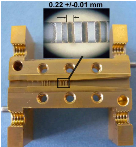
Fig. 21. LO band 2 134–184-GHz bandpass filter showing the detail of the machining precision, the WR6 input waveguide and the WR10 output waveguide. WR10 is the waveguide standard of the over-moded LO waveguide at the cryostat input.
