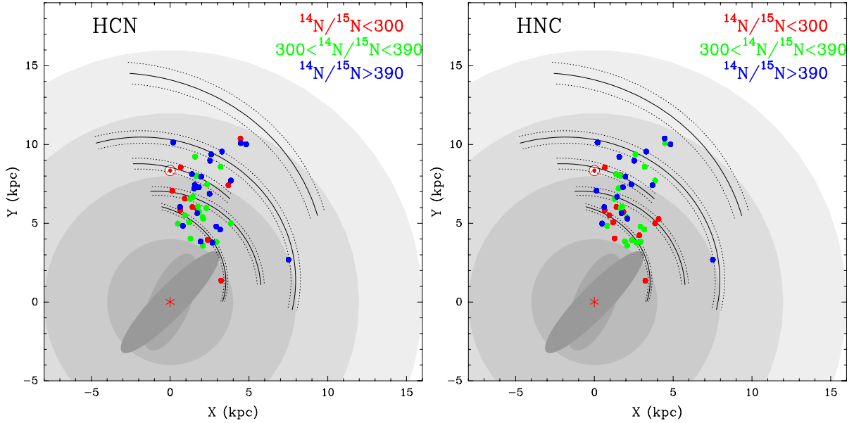
Figure 5. Plan view of the Milky Way. The Galactic center (red asterisk) is at (0,0) and the Sun (red Sun symbol) is at (0,8.34). The background grey discs correspond to the Galactic bar region (~4 kpc), the solar circle (~8 kpc), co-rotation of spiral pattern (~12 kpc) and the edge of major star-formation regions (~16 kpc). The solid black lines are the center of spiral arms traced by masers, and the dotted lines the 1\sigma widths. For more details see Reid et al. (2014). The filled circles represent sources of our sample implemented with those of Colzi et al. (2018), and the three colors are the ^{14}\text{N}/^{15}\text{N} ratios measured for HCN (left panel) and HNC (right panel): in red ^{14}\text{N}/^{15}\text{N} \leq 300 , in green 300 < ^{14}\text{N}/^{15}\text{N} \leq 390 and in blue ^{14}\text{N}/^{15}\text{N} \geq 390 .
