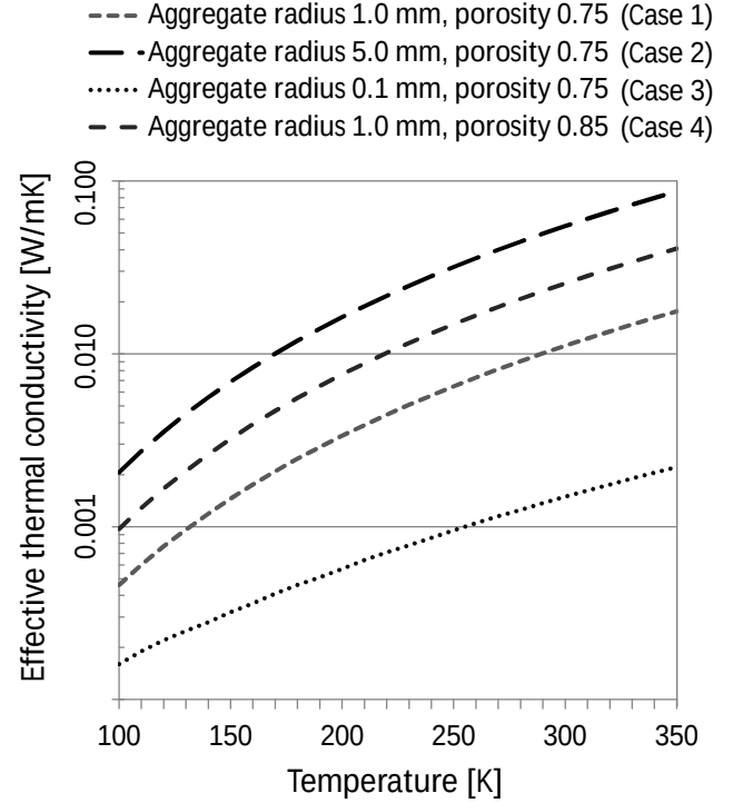
Fig. 4. Temperature-dependent effective thermal conductivities for thermophysical parameter cases 1-4: R denotes the radius of the agglomerates according to r_A in Table 4, case 4 assumes a high porosity of 85 % by lowering the fill factor of the agglomerate structure to 0.3. For comparison: lunar regolith is of the order of 0.001 W/mK.
