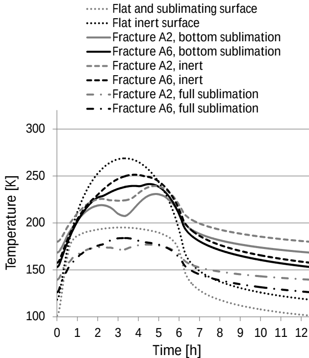
Fig. 17. Diurnal hemispherical brightness temperatures of flat and fracture geometries A2 and A6 for different sublimation patterns. The heliocentric distance is 2.0 AU, the plane angle is \eta = 30\text{deg} , and the sublimation front is identical to the surficial node. The dotted line shows the brightness temperature for flat terrains (sublimating and inert), while fracture geometries A2 (grey) and A6 (black) in three different configurations are displayed: for completely inert (dashed), sublimation of both bottom and walls (dash-dotted), and pure fracture floor/bottom sublimation.
