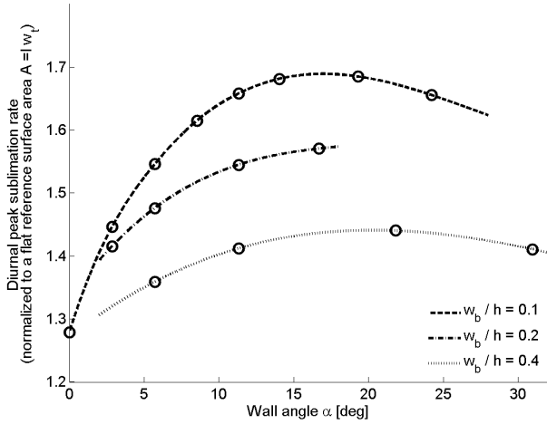
Fig. 8. Normalised peak sublimation rate as a function of fracture wall angle, analysed for 16 fracture geometries. The diurnal peak sublimation rate is normalised to that of a flat surface with identical illumination and thermo-physical properties, and the same area as the fracture bottom. The circles denote calculated values, the lines show interpolating cubic functions. The dashed line depicts fracture geometries A1-A8 with a bottom width-to-height ratio of 0.1, the dash-dotted line B1-B4 and the dotted line C1-C4. All calculations were performed for 2.0 AU heliocentric distance, a plane angle of 30 deg, and a surficial sublimation front.
