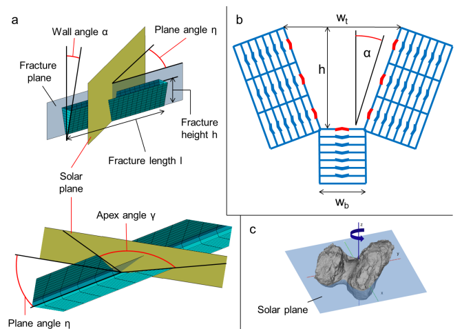
Fig. 3. Parametric model definition for a generic fracture: a) plane definitions, b) schematic nodal breakdown of a parametrised fracture with radiative heat exchange (red arrows) and effective conductive thermal fluxes (blue arrows), and c) solar plane with respect to the rotational axis of 67P at equinox.
