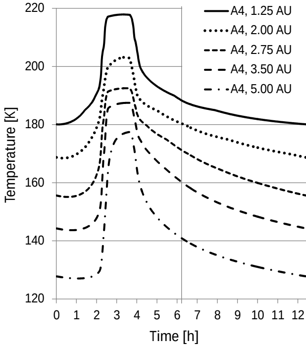
Fig. 13. Fracture A4 floor temperatures for five heliocentric distance settings with surficial sublimation. The vertical line at 6.2 h denotes the terminator.
