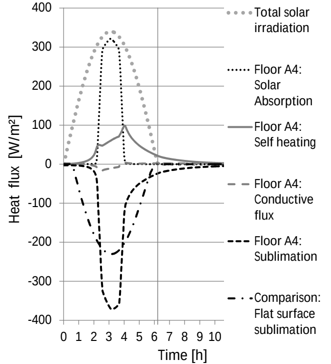
Fig. 5. Heat flux patterns for fracture A4 at a heliocentric distance of 2.0 AU and a plane angle \eta = 30 deg for one diurnal period of 12.4 h. The vertical lines at 0h and 6.2h indicate local morning and evening terminator. The coarse dotted grey line denotes the incident total solar irradiation, while the smaller black dotted line outlines the absorbed heat flux by the fracture floor. The grey continuous line shows the self-heating by infrared radiation, emitted from the fracture side walls, which impinges on the fracture floor: a positive value indicates a net heat flux direction towards the fracture floor. The grey dashed line illustrates the heat exchange with underlying nucleus layers through conductive and radiative transport. The black dashed line marks the local heat sink by sublimation phase change processes. For comparison, the dash-dotted line marks the sublimation pattern of a flat surface with identical thermophysical properties. The sublimation front is located directly at the surface of the coarse fracture floor. Remarks: (1) The heat fluxes are related to 1 m 2 sublimating fracture floor. Owing to the concave structure of geometry A4 and the decreasing width with depth, the fracture top sums up to 4 m 2 . (2) The fractured terrain absorbs about 4 % more thermal energy than a flat surface because scattered irradiation is absorbed.
