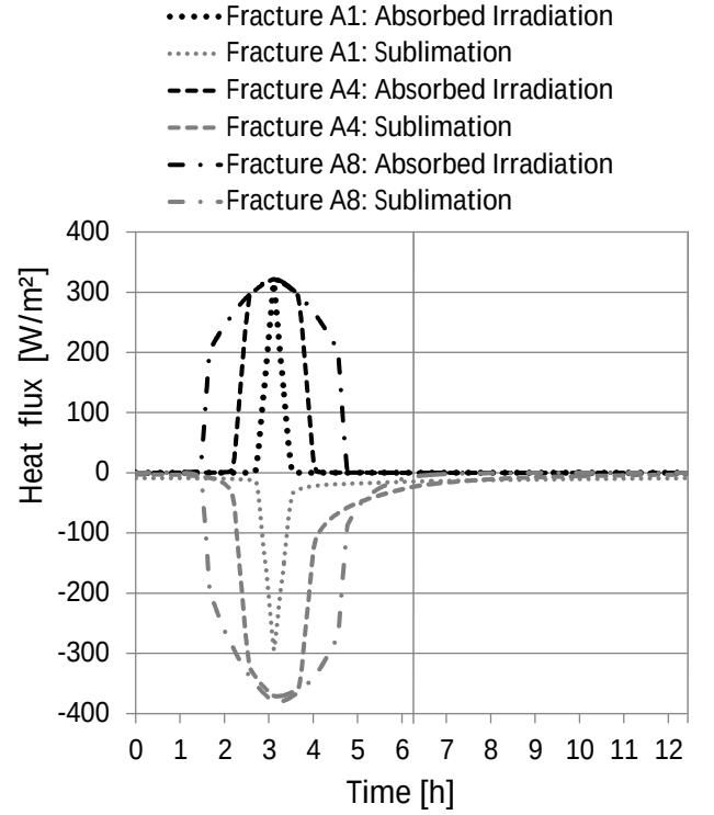
Fig. 7. Diurnal absorbed solar irradiation and sublimation fluxes for fractures A1, A4, and A8. The fracture floor sublimation front is located directly at the surface node. The vertical line at 6.2h denotes the evening terminator.
