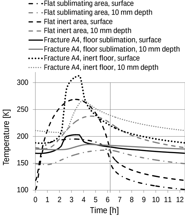
Fig. 6. Calculated diurnal temperatures for flat terrain and for the bottom of fracture geometry A4. The heliocentric distance is 2.0 AU, the plane angle is \eta = 30 deg, and the sublimation front is identical with the surface. The displayed fracture temperatures are averaged values over the four most central node positions at the fracture bottom, and 10 mm below it.
