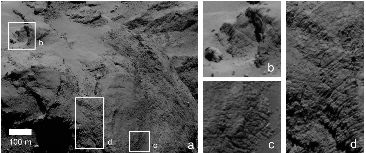
Fig. 1. Selected fractured areas on comet 67P/Churyumov-Gerasimenko, on Image NAC_2014-09-14T16.21.40.802Z_ID30_1397549001_F41. a) Overview of the Ma'at regional morphology, according to El-Maarry et al. (2015a) b) Fractures at the tops and sides of escarpments or cliffs. c) Fracture networks. d) Fractures on inclined terrain, grouped with similar-width orientation. See El-Maarry et al. (2015b) for the abundance and classification of fracture morphologies.
