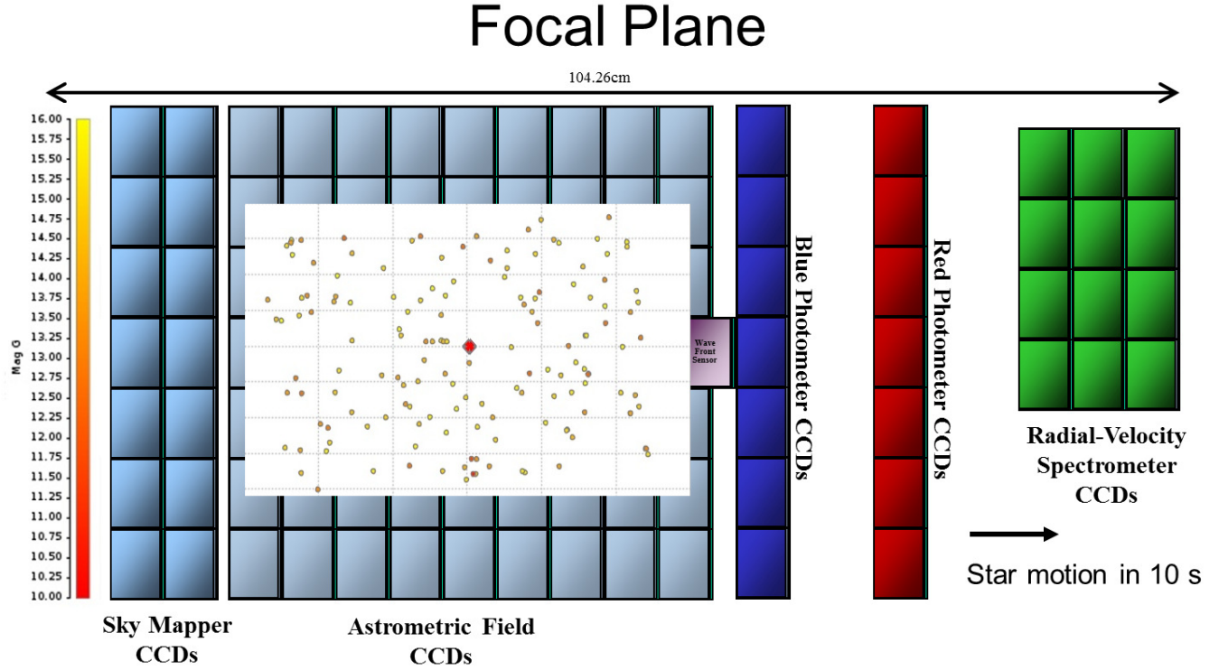
Figure 3. The Gaia focal plane showing the Astrometric, Red and Blue Photometers and RV Spectrometer alongwith the SkyMapper. The star field of interest is superposed on the focal plane and shows stars with G < 16 mag in a window of size 0.6 \times 0.4 degrees around the north ecliptic pole shown in red and roughly in the middle of the Astrometric Field, i.e. the fifth CCD column, where each grid size is 0.1 degrees in the x-direction and 0.05 degrees in the y-direction. The stars are colour-coded according to their magnitudes given by the vertical colour bar shown on the left. Background image credit: ESA - A. Short.
