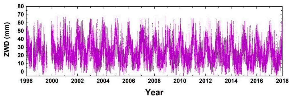
Figure 3. Hourly Zenith Wet Delay estimated at Casey Antarctic station.
