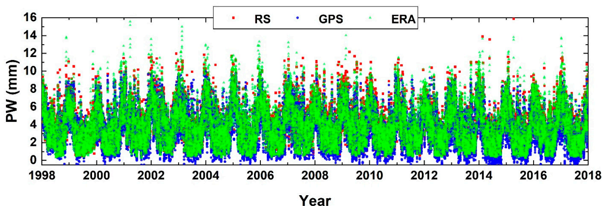
Figure 6. PW time series in mm for Casey: from RS (red circles), from GPS (blue squares) and from ERA (green triangles).
