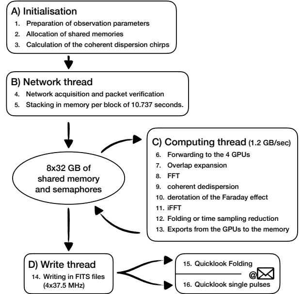
Fig. 3. Operational scheme of the LUPPI pipeline, including its main elements: initialization (A) of the observation parameters, the data processing cycle organized in threads around a shared memory and communicating through semaphores, and post-processing of the observation with production of “quicklook” plots. The network thread (B) catches the packets sent by the beamformer, the computing thread (C) processes the data in the Fourier domain on GPUs, and the write thread (D) exports data products to disks.
