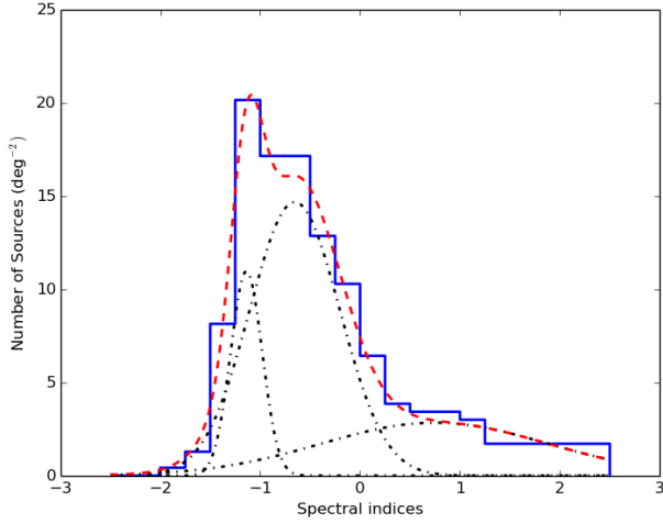
Figure 7. Spectral index distribution of the SCORPIO survey using a 0.25 wide bin in blue straight line, modeled using 3 Gaussians (red dashed line). In black dash-point line the three Gaussian components of the final model.
