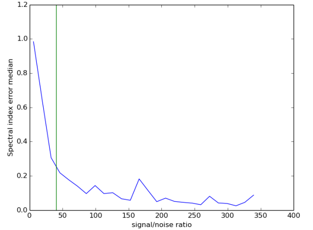
Figure 6. The median on the spectral indices error against S/N in SCORPIO. The green line indicates the 40\sigma limit.
