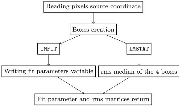
Figure 1. Flowchart for the flux density extraction algorithm
