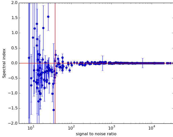
Figure 5. Spectral indices against S/N in the simulation. All the sources have been built to have a flat SED, but the spectral indices are not accurate enough below 40\sigma (indicated by the red line).
