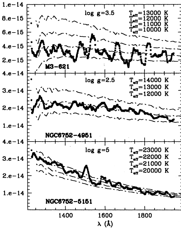
Fig. 3. Comparison of the spectral energy distributions of the stars 621 in M 3, and 4951 and 5151 in NGC 6752, with the Kurucz (1992) model atmospheres (dashed lines) corresponding to the values of gravity and temperature indicated in each panel
