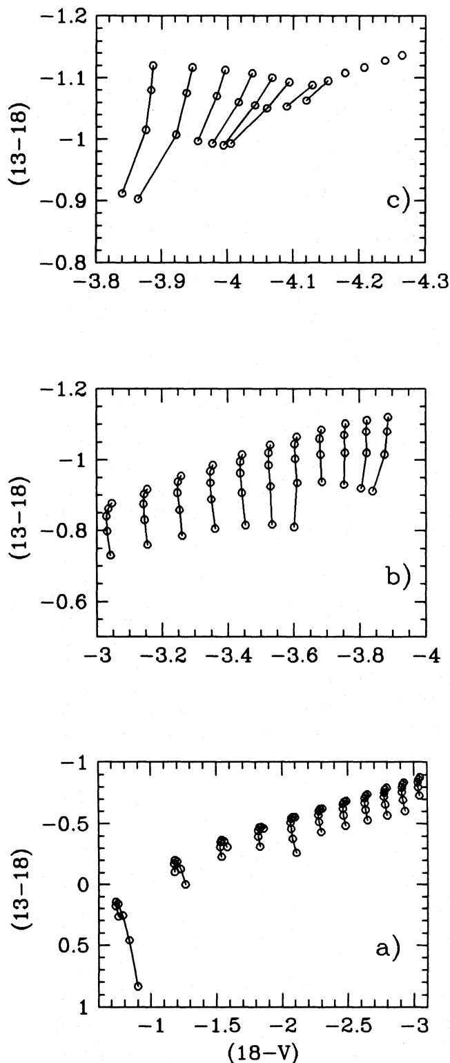
Fig. 2a–c. UV colours (13–18) vs. (18–V) from K92 model atmospheres with [m/H] = -1.5 . The solid lines connect the models at a given temperature and different gravities decreasing from \log g = 5.0 (top dot) in steps of 0.5. For the sake of clarity the models have been plotted in three temperature ranges: a from 10,000 to 20,000K in steps of 1,000K, left to right; b from 20,000 to 30,000K in steps of 1,000K; c from 30,000 to 35,000K in steps of 1,000K, and from 35,000 to 50,000K in steps of 2,500K
