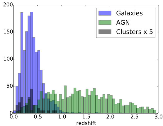
Figure 4. A redshift histogram of AGN, clusters (scaled by x5) and galaxies in the XXL southern field. The AGN extend out to z \sim 5 , and the clusters out to z \sim 0.9 . Not shown are the 44 AGN in the redshift interval 3 \leq z \leq 5 .
