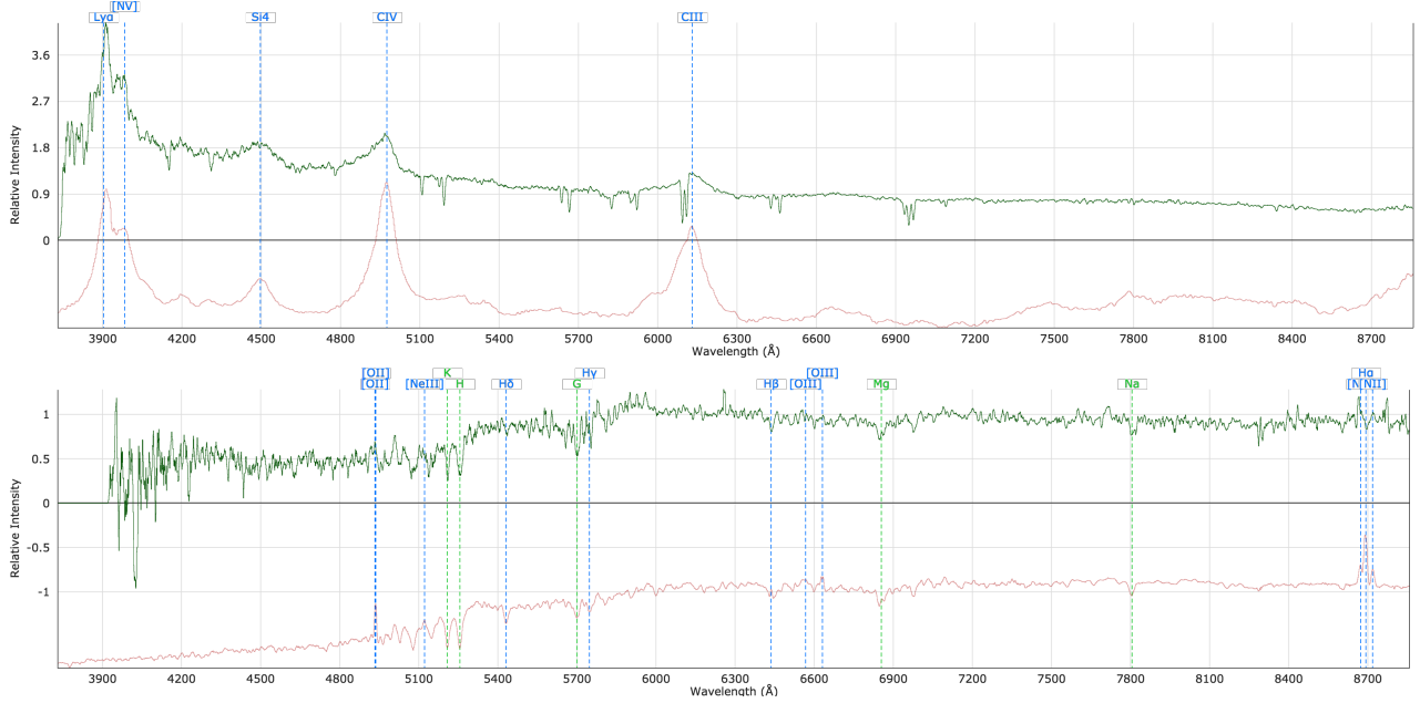
Figure 3. Sample spectra (in green) showing an AGN with broad emission lines (above) and a cluster galaxy (below). Template spectra are shown in red. The vertical lines mark commonly observed lines in AGN and galaxies. This plot was produced using the output from Marz (Hinton et al. in preparation).
