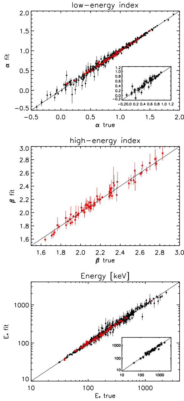
Fig. 3 Best-fitting spectral parameters (low-energy spectral index \alpha , upper panel, high-energy spectral index \beta , middle panel, and characteristic energy E_0 , lower panel) for the cutPL (black points, 446 GRBs) and Band (red squares, 73 GRBs) functions, compared to the “true” values used to simulate the spectra with the ECLAIRs+GRM system. The solid lines mark the equality. The same quantities for the 50 short GRBs are portrayed in the insets.
