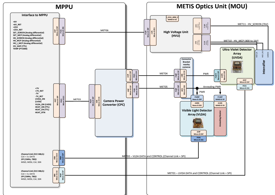
Data from the camera is transferred via a channel link interface to the Metis Power and Processing Unit (MPPU) and a separate SPI interface is used for commanding and housekeeping. The power is provided by the MPPU through a Camera Power Converter (CPC), which converts the primary output voltage from the MPPU to the supply voltages for the VLDA and UVDA cameras. The voltages required by the MCP and the phosphor screen are provided by a High Voltage Unit (HVV) mounted on the S/C panel at the side of the Metis telescope. Figure 2 shows a block diagram of Metis electronics system.
