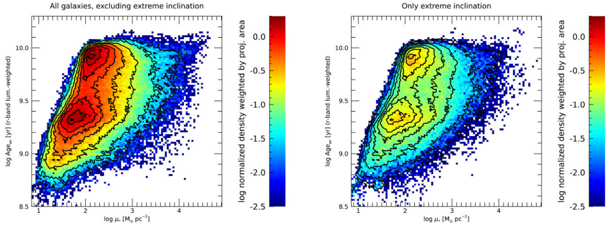
Figure B1. Distribution of galaxy regions, volume corrected and weighted by physical projected area, in the \log \mu_* – \log \text{Age}_w plane: contours display the distribution for the full galaxy sample (same as Fig. 6), while the colours show the distributions after excluding high inclination systems (left panel) and for highly inclined disks only (right panel). Note: the sum of these two distributions is exactly the distribution of Fig. 6.
