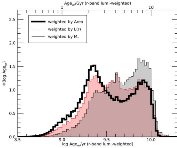
Figure 2. Distributions in r -band luminosity weighted age, \Phi(\log \text{Age}_{\text{wt}}) , for all regions in all galaxies, weighted by physical projected area, r -band luminosity and present-day stellar mass, respectively (see legend). All distributions are corrected for V_{\max} and normalized to unity integral.
