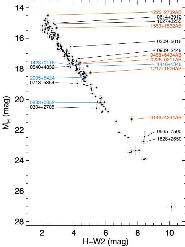
Figure 8. Trends of absolute H -band magnitude with H -W2 color for all objects from Table 7 that fall within 20 pc of the Sun ( \pi_{\text{abs}} \geq 50 mas). Known binary systems are circled and labeled in red, and known subdwarfs are circled and labeled in blue. Other objects falling significantly above or below the mean trend are labeled in black.
