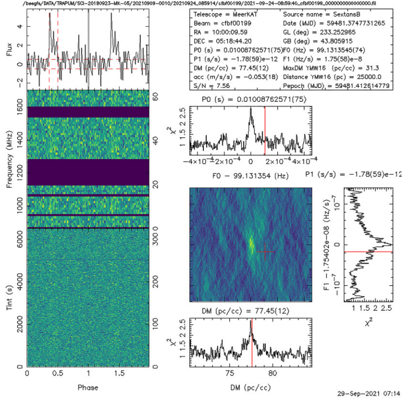
Figure 3. An example of a low-confidence candidate from this survey, from the third pass observation of Sextans B. Details of the PULSARX folding package can be found in Men et al. (2023).
