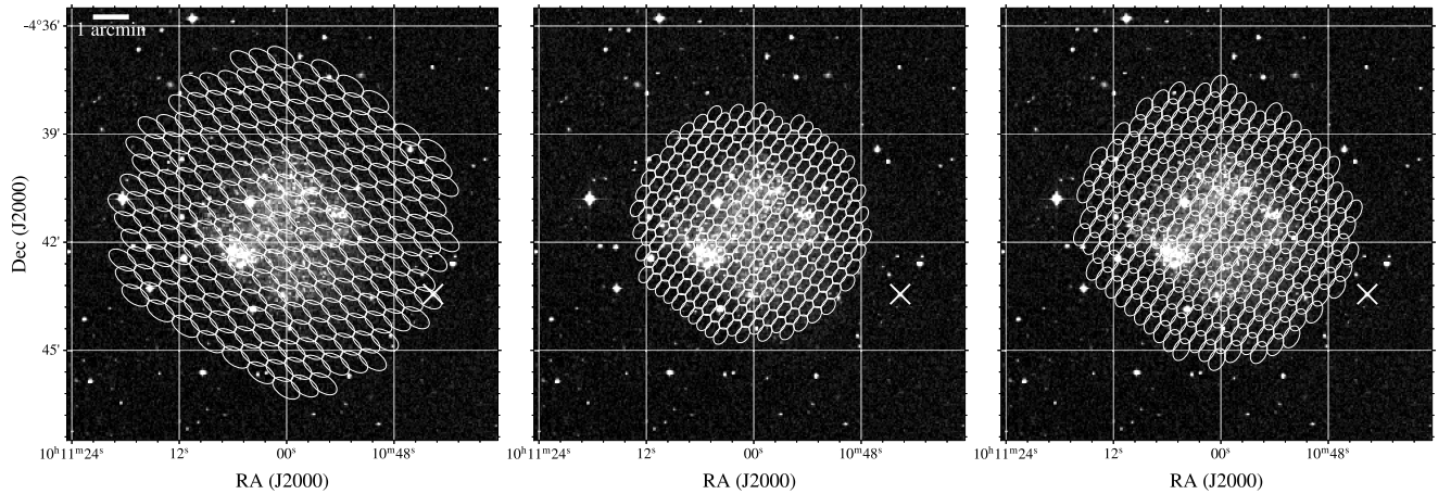
Figure 1. The three observations of Sextans A (first to third pass left to right) are displayed over a DSS image (Space Telescope Science Institute 1995). The observed MeerKAT full array coherent beams are shown at 50 per cent sensitivity (47 per cent for the first pass) as white ellipses, simulated with MOSAIC. The MeerKAT incoherent beam size is larger than the figure with a FWHM of about 1 deg at L band. This figure was generated with the (0:sc)aplypy/(0:sc) Python package. The GC (Beasley et al. 2019) is shown with a cross. The beam orientation changes are due to the source being observed when rising in the first pass and setting in the two other passes. The beam size depends on the hour angle of the source and the location of the antennas used.
