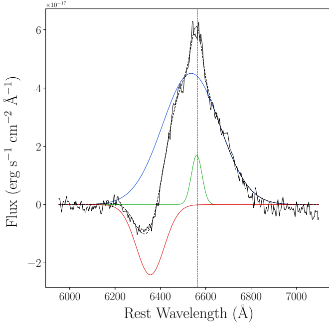
Figure 14. The H\alpha profile +132d described by a combination of three Gaussian profiles, representing a P-Cygni profile as well as an intermediate width feature with FWHM \sim 2700 km s ^{-1} at the rest wavelength of H\alpha . The broad H\alpha emission is blueshifted by \sim 1100 km s ^{-1} . A linear fit to the continuum has been subtracted from the data.
