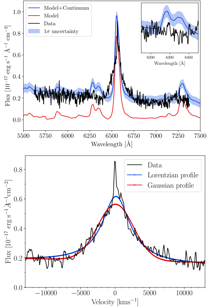
Figure 11. Upper panel: The +301 rest frame day spectrum of SN 2016gsd, shown in black, as compared to a model of the nebular spectrum obtained for the explosion of a 15 M_{\odot} ZAMS red supergiant at +306d, shown in red (Jerkstrand et al. 2014). The model flux has been scaled to correspond to the distance of SN 2016gsd. In blue we show the model with the addition of the continuum found in the data. The shaded region shows the uncertainty derived from the data and applied to the model. The inset shows the region around the [O I] \lambda 6300, 6364 emission lines. Lower panel: H\alpha line profile in velocity space, with the best fit broad Lorentzian profile overplotted in blue, and the broad Gaussian profile in red.
