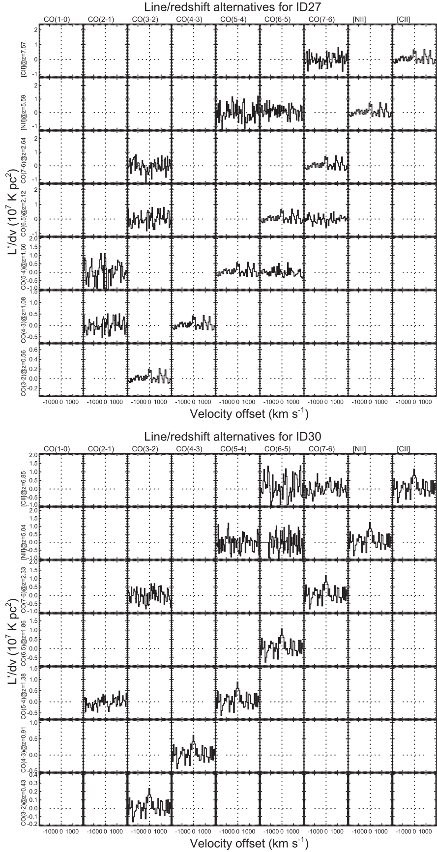
Figure 18. Line identification for the optical dropout galaxies associated with a 1 mm line candidate, ID27 and ID30. Each row represents the identification of an emission line and redshift. For each row, the different cells show the spectra around other lines covered by our 3 mm and 1 mm scans at the identified redshift. As expected for distant z > 6 galaxies, the only line identified corresponds to [C II], and other lines, such as CO(6-5), CO(7-6), or CO(8-7), are too faint to be detected by our 3 mm scan.
