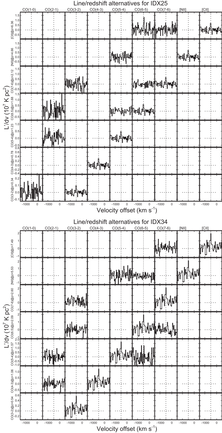
Figure 15. Line identification for the blind [C II] line candidates with no optical association, IDX25 and IDX34. Each row represents the identification of an emission line and redshift. For each row, the different cells show the spectra around other lines covered by our 3 mm and 1 mm scans at the identified redshift. As expected for distant z > 6 galaxies, the only line identified corresponds to [C II], and other lines, such as CO(6-5), CO(7-6), or CO(8-7), are too faint to be detected by our 3 mm scan.
