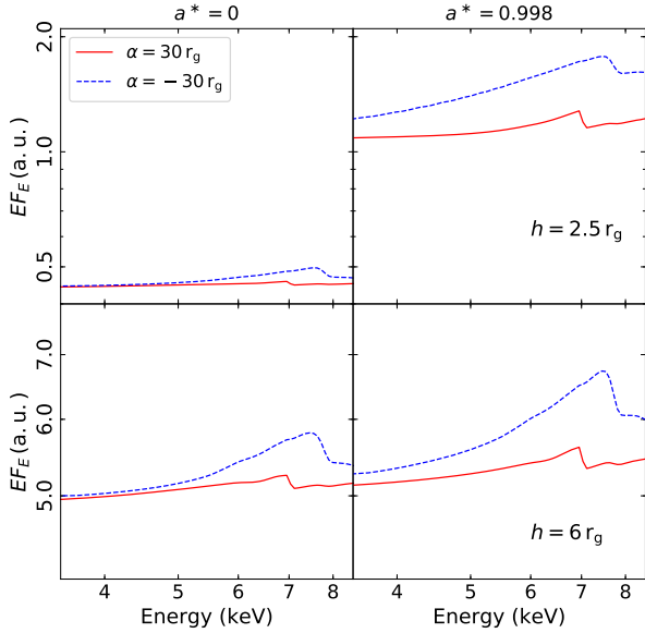
Figure 3. The observed spectra, in the 3.5–8.5 keV range, considering a cloud of radius 30r_g obscuring the approaching ( \alpha = 30r_g , solid red lines) and receding ( \alpha = -30r_g , dashed blue lines) parts of the accretion disc for BH spins of 0 (left panels) and 0.998 (right panels). We consider primary sources located at 2.5 and 6 r_g (top and bottom panels, respectively) above an accretion disc with an inclination of 60^\circ .
