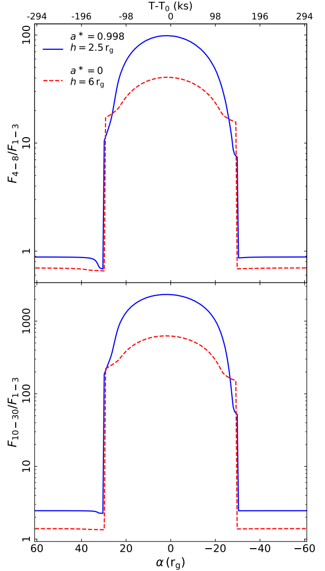
Figure 4. Examples of the hard-to-soft flux ratios expected from X-ray eclipses by a cloud of radius 30r_g , as it moves along the line of sight. We consider the soft band in the 1–3 keV range as a proxy of the primary emission, and two hard bands the 4–8 (top panel) and 10–30 keV (bottom panel) bands, which should be dominated by the FeK line and the Compton hump, respectively. We show the cases of a maximally rotating BH with a lamp-post located at 2.5 r_g (solid blue lines) and a Schwarzschild BH with a lamp-post located at 6 r_g (dashed red lines).
