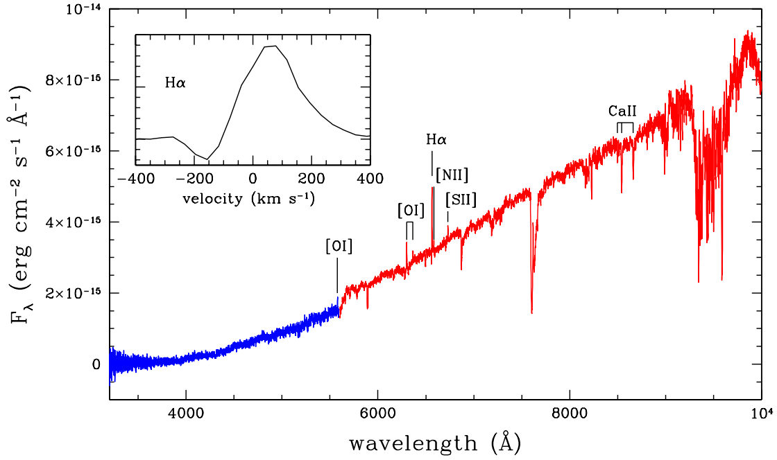
Fig. 2. LBT/MODS spectrum of V1184 Tau. Blue and red channels spectra are depicted with the corresponding color. Main features are labelled. In the insert we show the H \alpha spectral profile.
