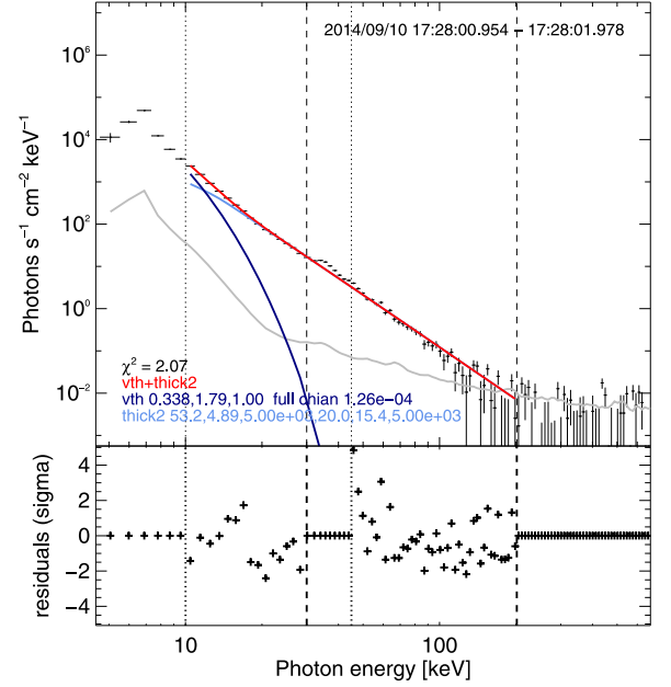
Figure 8. Top panel: HXR spectrum around the time of flare maximum, from Fermi-CSPEC data (black points with error bars). In gray we plot the preflare background flux averaged between 17:13 and 17:15 UT. The colored curves represent the fit obtained from the OSPEX forward-fitting procedure, including a thermal component (dark blue), a single power-law component (light blue), and the combined fit (red). Dotted and dashed lines indicate the lower and upper limits of the two energy ranges used for the nonthermal component fit (10–30 keV and 45–200 keV); this is necessary because of calibration issues that affect the intermediate energies (see the text). Bottom panel: the residuals between the fitted distribution and real data, normalized to the 1\sigma uncertainty for each respective data point. The fitted distribution can be considered acceptable because most of the points lie within 2\sigma .
