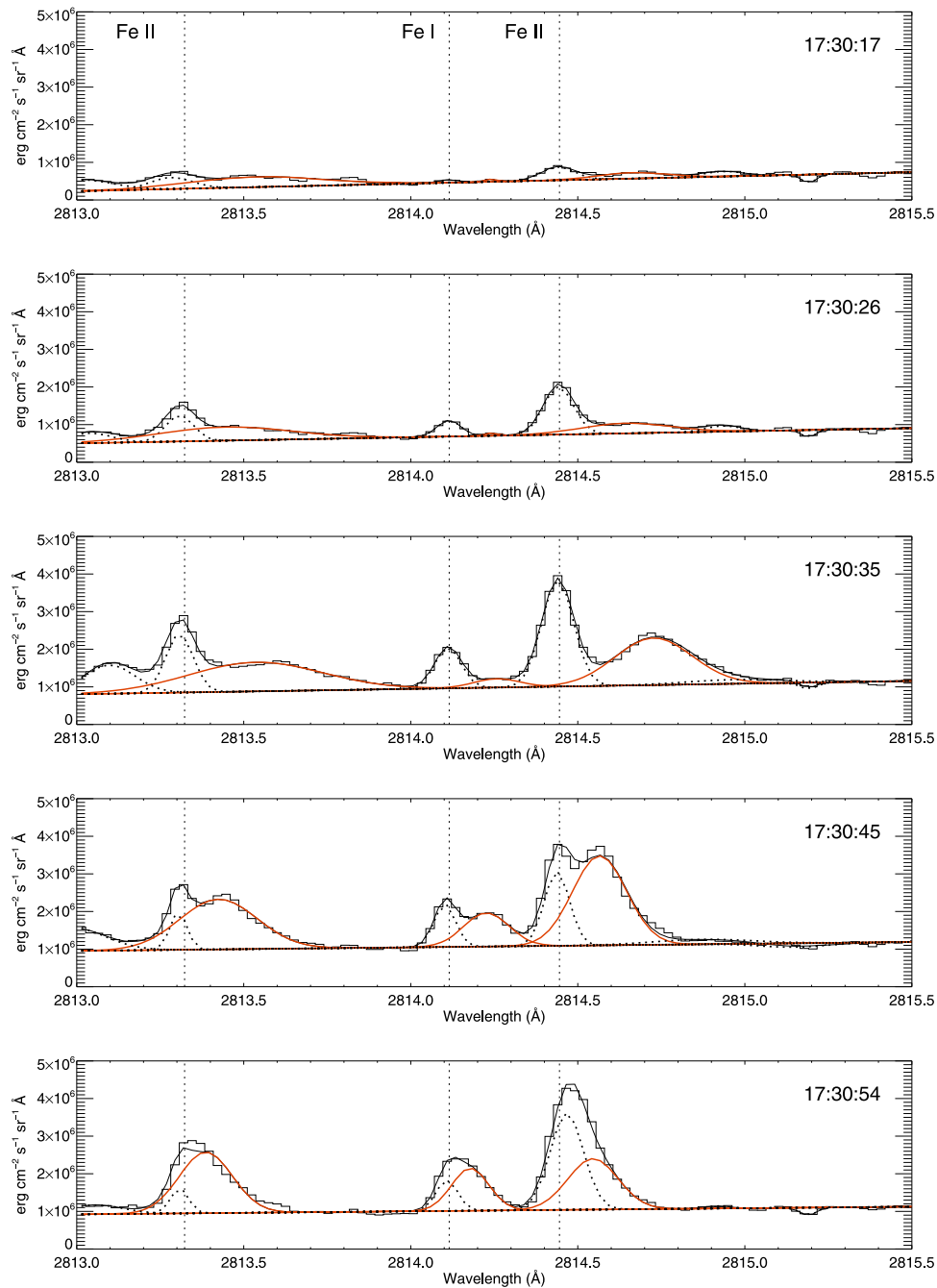
Figure 5. Temporal evolution of the spectra in the Fe II window for multiple chromospheric lines (stepped black lines) for the y = 119''/53 slit pixel (see markings in Figure 1). The dotted vertical line represents the rest wavelength for each line (labeled in the top panel). Dashed black lines represent the Gaussian fits for the stationary component; red lines the fit for the redshifted components, and the total fit is given as a solid black line. Note that the Gaussian fits are displayed at the native resolution of the IRIS spectra. Time runs vertically, corresponding to the red diamonds in Figure 4 (successive exposures at the overall 9.4 s cadence; 2.4 s exposure). The intensity scale is kept constant to better appreciate the variations in brightness during the flare. No subtraction of preflare background has been performed.
