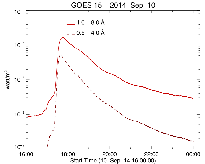
Figure 2. GOES 1–8 Å flux over several hours around the event. The data used in this paper pertain to the very rapid impulsive phase, as framed by the dashed lines.
