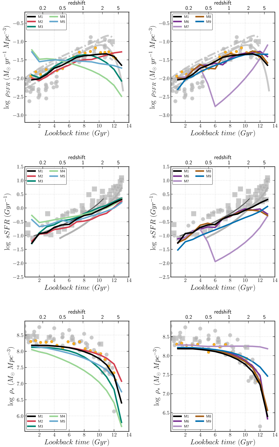
Fig. A.5. Cosmic evolution of SFR ( \rho_{\text{SFR}} , upper panels), sSFR (middle panels), and stellar mass ( \rho_* , bottom panels) for one single parametric SFH (left panels) and a combination of two parametric SFH (right panels). The reference delayed- \tau model (M1, black line) is plotted in all the panels. Gray and yellow points and gray curves are taken from the literature as explained in the text and in the captions of Figs. 6–8.
