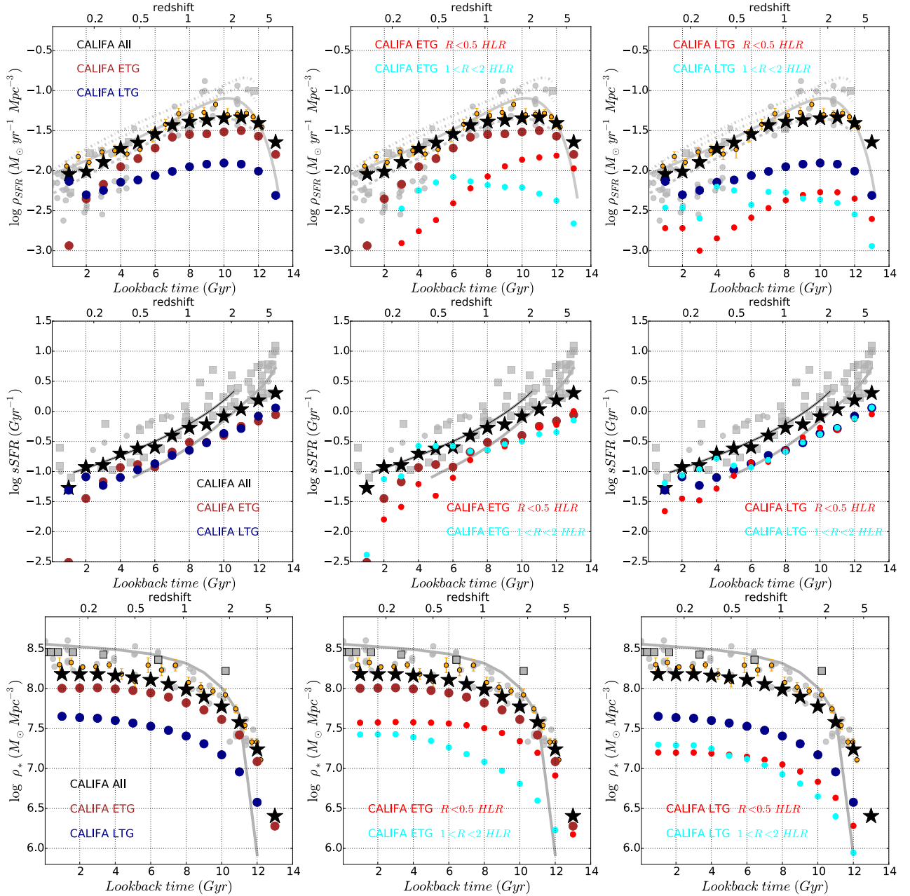
Fig. 10. Cosmic evolution of the SFR density, \rho_{\text{SFR}} (upper panels), the \text{sSFR}(t) (middle panels), and the stellar mass volume density, \rho_* (lower panels) as a function of the morphology: early-type (E, S0, and Sa) and late-type (Sb, Sbc, Sc, and Sd) galaxies. The contribution of the inner ( R < 0.5 HLR) and outer ( 1 < R < 2 HLR) regions of ETGs and LTGs are listed in the central and right panels, respectively.
