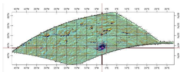
Fig. 3: Color composite of VIR normalized data (Red: 1.86 \mu\text{m} ; Green: 2.00 \mu\text{m} ; Blue: 2.18 \mu\text{m} ). The blue unit illustrates the negative spectral slope of high-albedo materials within crater Oxo. H 2 O-rich materials are only two pixels within this blue unit.
