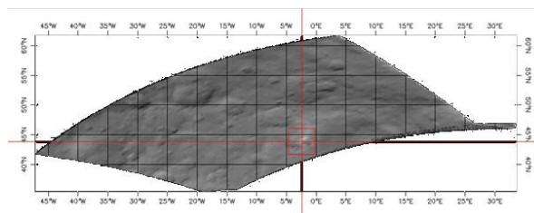
Fig. 2: I/F image at 1.1 \mu\text{m} that shows the first observation of crater Oxo by the VIR imaging spectrometer during Dawn's Survey orbit around Ceres. The red lines cross at the location of the H 2 O detection (only two pixels in this image).
