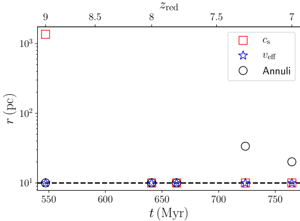
Figure 14. Influence radius of the MBH in our simulation at z = 9, 8, 7.8, 7.3 , and 7 , estimated as the Bondi radius (red squares), the Bondi-Hoyle-Lyttleton radius (blue stars), and by comparing the Keplerian velocity due to the MBH to the rotational velocity and velocity dispersion of the gas around it (black circles). Apart from some deviations, in particular at high redshift for the Bondi radius, and around z = 7 - 7.3 for our third estimator, the radius is always comparable to the spatial resolution of our simulation, hence likely unresolved in current and upcoming observations.
