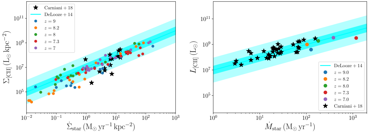
Figure 13. [CII]–SFR relation in our simulation (as dots, colour-coded by redshift), compared with the low-redshift sample by De Looze et al. (cyan shaded areas, corresponding to 1\sigma (darker) and 3\sigma scatter (lighter) 2014) and the high-redshift data by Carniani et al. (black stars 2018). The left-hand panel corresponds to the resolved relation, estimated by binning the 2D flux maps in 300 pc patches, whereas the right-hand one to the integrated relation. Our results show that, despite small fluctuations of the data relative to the relation at higher redshift, the quasar host well settles on the local relation (either resolved or integrated) and is also in good agreement with the high-redshift galaxies by Carniani et al. (2018).
