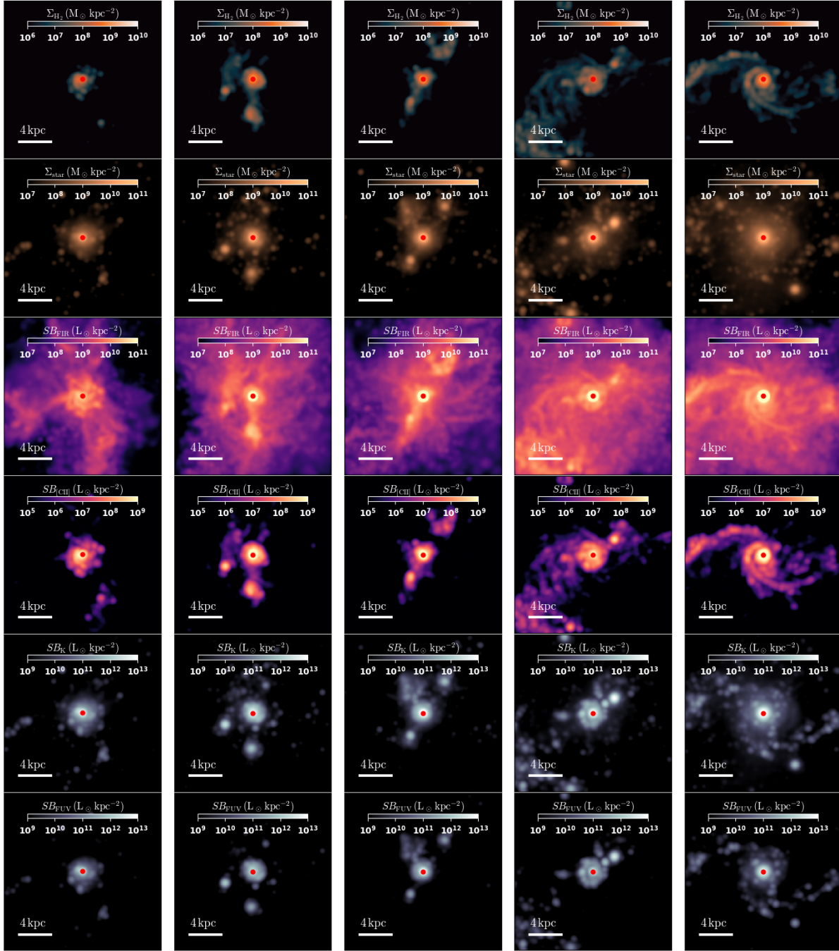
Figure 12. Same as Fig. 10, degraded at 500 pc resolution. Unlike for the 2 kpc case, here most of the features are still visible, simply spread over a larger area. Such features may be potentially observable by current and upcoming facilities like ALMA and JWST, provided a long enough integration time.
