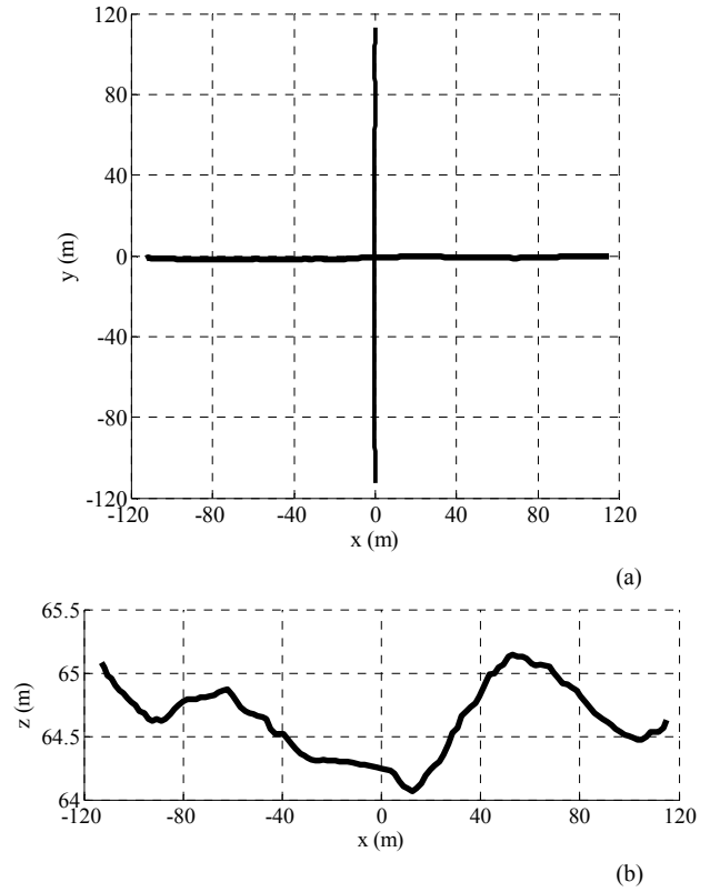
Fig. 3. (a) Flight paths projected on the horizontal plane, (b) flying height during the scan along the x -axis. The position data are measured by the differential GNSS receiver.
