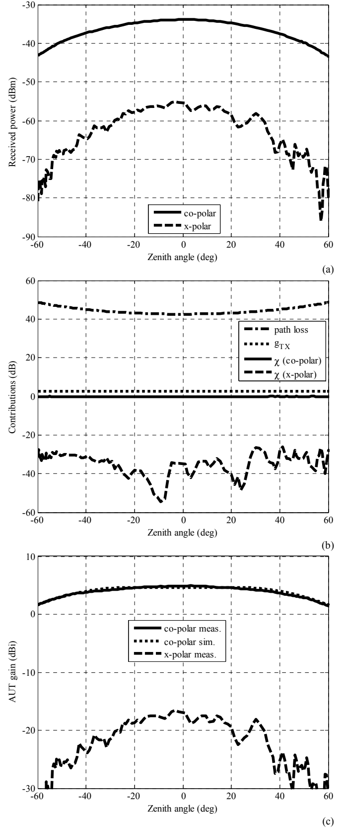
Fig. 6. (a) Received power pattern, (b) contributions of the Friis formula, (c) extracted AUT radiation pattern.
