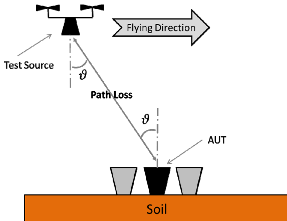
Fig. 2. Illustration of an embedded-element radiation pattern measurement.
