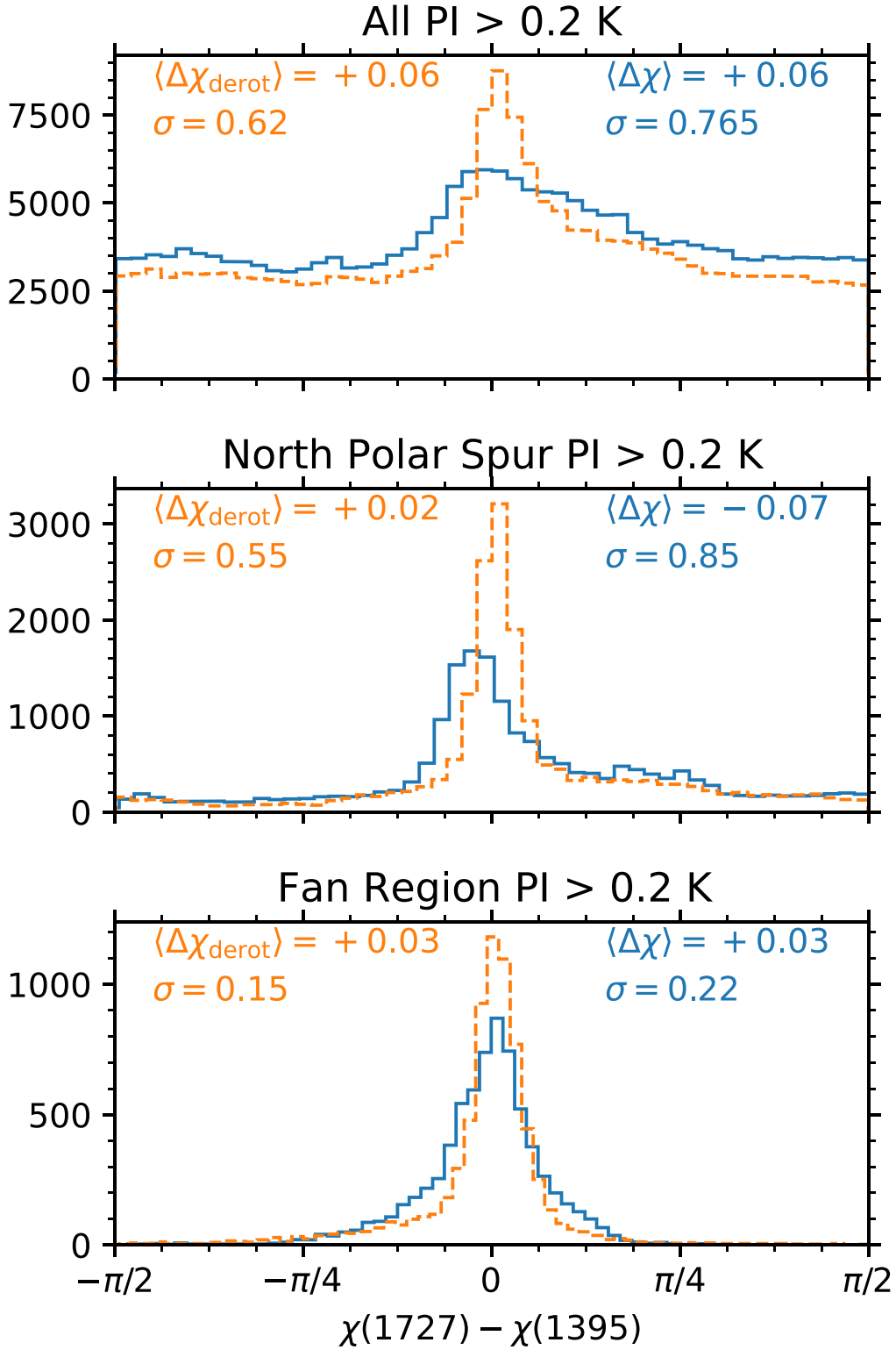
Figure 18. Histograms of the differences in polarization angle for the scatter plots of Figure 17. The mean, \langle \Delta \chi \rangle , and standard deviation, \sigma , for each histogram are indicated.
