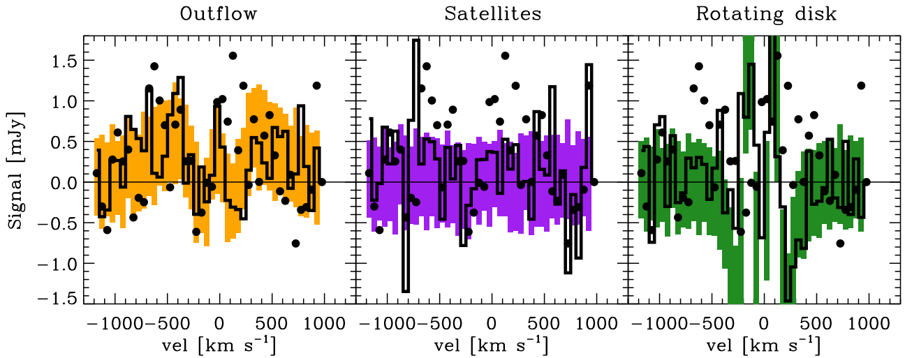
Figure 5. Combined residuals for the synthetic samples (see the left-hand panel of Fig. 2). Filled black circles refer to the C15 sample. The black thick lines represent the realizations that provide the best agreement with data, while the coloured shaded regions quantify the 1\sigma dispersion over the 500 realizations.
