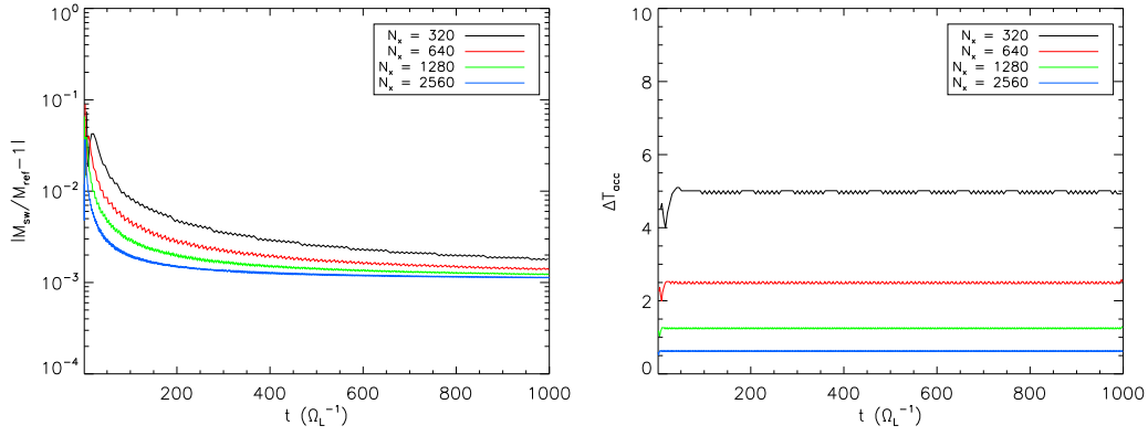
Figure 7. Left panel: relative error |M_{\text{sw}}/M_{\text{ref}} - 1| of the cumulative swept mass as a function of time, where M_{\text{sw}} = \Delta x \Delta y \int_0^t \sum_i (\rho_{\text{sh}})_i while M_{\text{ref}} = \rho_0 v_{\text{sh}} t L_y is the expected value for a 1D plane-parallel shock. Right panel: duration of an accumulation cycle as a function of time. Colors correspond to different grid resolutions reported in the legend.
