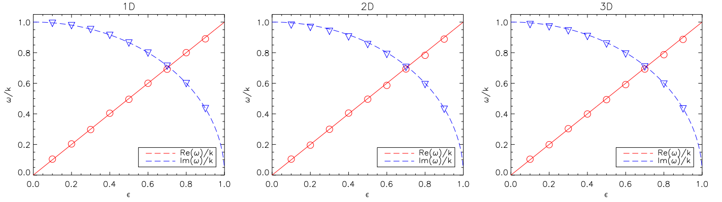
Figure 5. Real (red) and imaginary (blue) parts of the growth rate for the nonresonant Bell instability problem using different values of the \epsilon parameter. The solid and dashed lines give the theoretical expectation, Equation (66), while the symbols (triangles and circles) are the results measured from the simulations using the CTU scheme.
