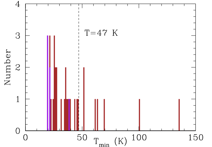
Fig. 3. Distribution of the minimum blackbody temperature T_{\min} required to explain the observed 1.2 mm brightness of z \sim 6 QSOs. The Venemans et al. (2020) and SHELLQs samples are shown in brown and purple, respectively. Note that the 1.2 mm emission on approximately kiloparsec scales of a few bright objects can only be reproduced by hot dust with T_d > 50 –100 K. We used T_d = 47 K, a standard reference value used in the literature (e.g., Venemans et al. 2020), to derive the dust masses of all QSOs with T_{\min} < 47 K. For hotter systems, we used T_d = 1.2T_{\min} (see text for details).
