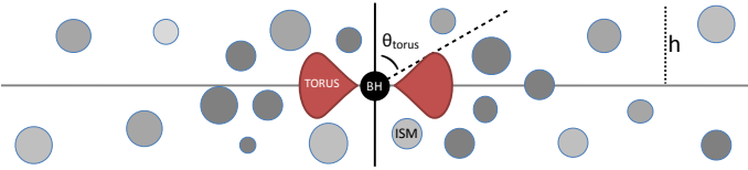
Fig. 12. Edge-on view of the considered geometry for the ISM clouds and the torus (not to scale).
