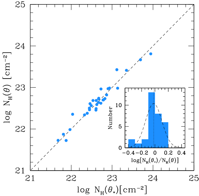
Fig. 6. Comparison between the ISM column densities toward the nucleus of ASPECS galaxies derived by assuming a fixed, average galaxy orientation ( \theta_* = 57.3^\circ ) vs. those derived from individual galaxy orientations \theta . The inset shows the distribution of the \Delta \log N_{\text{H,ISM}} values: a Gaussian fit (dashed curve) is centered at about 0 (dotted line) and has rms \sim 0.15 dex.
