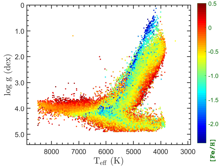
Fig. 5 Kiel diagram ( \log g vs. T_{\text{eff}} ) of the “qualified” LK spectra. The parameters are derived from the LK pipeline. Note that different colors indicate different values of metallicity [\text{Fe}/\text{H}] .
