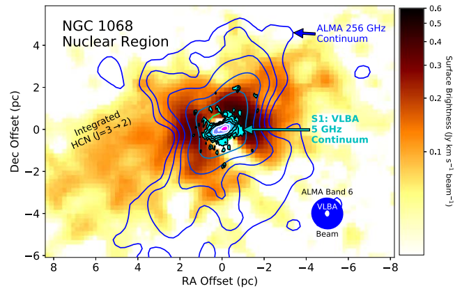
Figure 1. Nuclear region of NGC 1068 shown as overlays of the ALMA 256 GHz continuum (blue–green unfilled contours; Band 6), VLBA 5 GHz continuum (black contours filled with shades of cyan to magenta; Gallimore et al. 2004), and ALMA integrated HCN ( J = 3 \rightarrow 2 ; Band 6; background image in shades of yellow to dark red). A compact source model for S1 has been subtracted from the ALMA continuum; the flux density of the compact source is 6.6 \pm 0.3 \text{ mJy} . The Band 6 contour continuum levels are (blue) 0.019, 0.037, 0.075, 0.15, (blue–green) 0.30, and (green, mostly obscured by the VLBA continuum contours) 0.60 \text{mJy beam}^{-1} . The integrated HCN image is shown with an arcsinh stretch and surface brightness limits 0.004 ( 5\sigma ) to 0.6 \text{ Jy km s}^{-1} \text{ beam}^{-1} . Blanked values ( < 5\sigma ) display as white.
