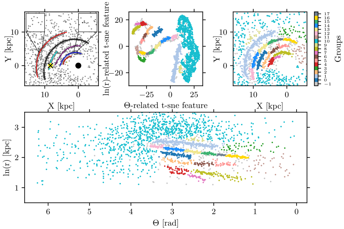
Fig. B.7. Same as Fig. B.1, but with random noise added to the (x,y) coordinates of the N_{\text{spiral}}=900 stars in the mock spiral arms, and N_{\text{other}}=1500 inter-arms' Cepheids.
