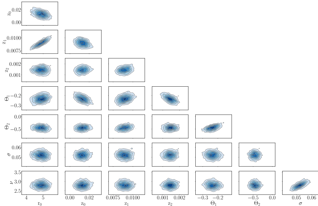
Fig. A.2. Pairwise correlations of the posterior distributions of the structural parameters r_0 , z_0 , z_1 , z_2 , \Theta_1 , \Theta_2 of the warp model, together with the standard deviation \sigma and the normality parameter \nu of the model.
