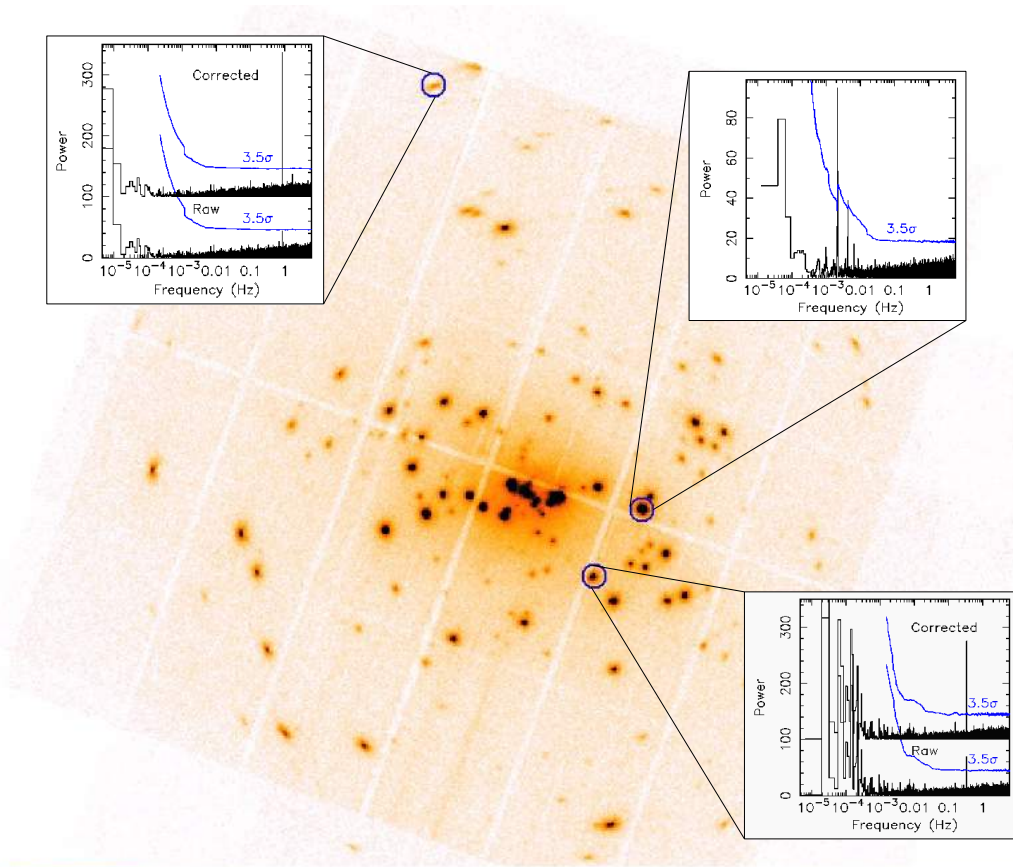
Fig. 18. XMM pn plus MOSs cleaned image of ObsId 0112570101 (64 ks effective exposure time) for the galaxy M31. The insets show the pn power spectra (solid black lines) together with the local 3.5\sigma detection threshold (solid blue lines) obtained from the unbinned event lists of the three pulsating sources discovered during the EXTras project and discussed in Sect. 4.6: J004301 (ObsId 0505720301), J004222 (ObsId 0600660401, 0600660501, and 0650560601 together) and J004232 (ObsId 0764030301) from top to bottom. In the cases of J004301 and J004232, the discovered X-ray pulsars revolve around a companion star. In the corresponding insets we show the power spectra with (corrected) and without (raw) the best inferred orbital corrections (shifted by 100 in power on the y-axis for clarity).
