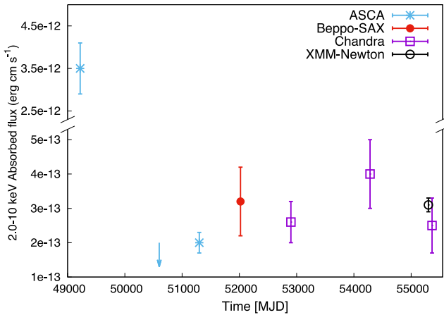
Figure 6. Absorbed 2–10 keV light curve of AX J184453–025640. The ASCA, BeppoSAX, and 2003 Chandra fluxes are taken from Tam et al. (2006). The BeppoSAX and ASCA fluxes might be overestimated due to the presence of other unresolved sources.
