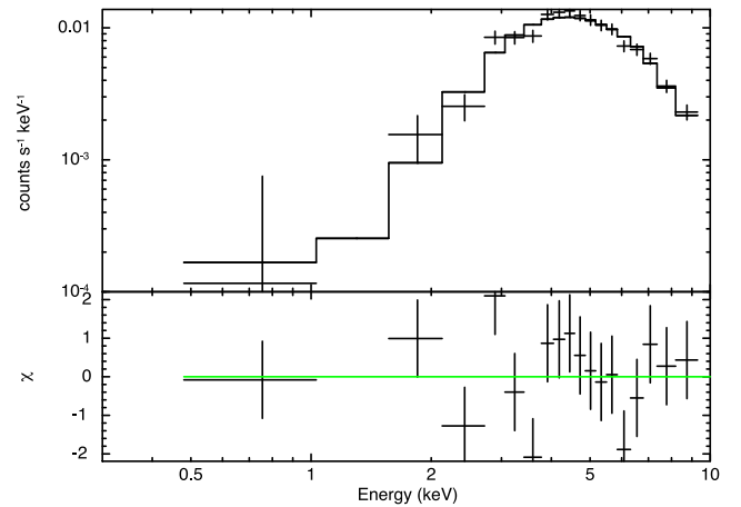
Figure 2. EPIC spectrum of AX J184453–025640 (source F). Top panel: data and best-fitting power-law model. Bottom panel: residuals in units of \sigma .
