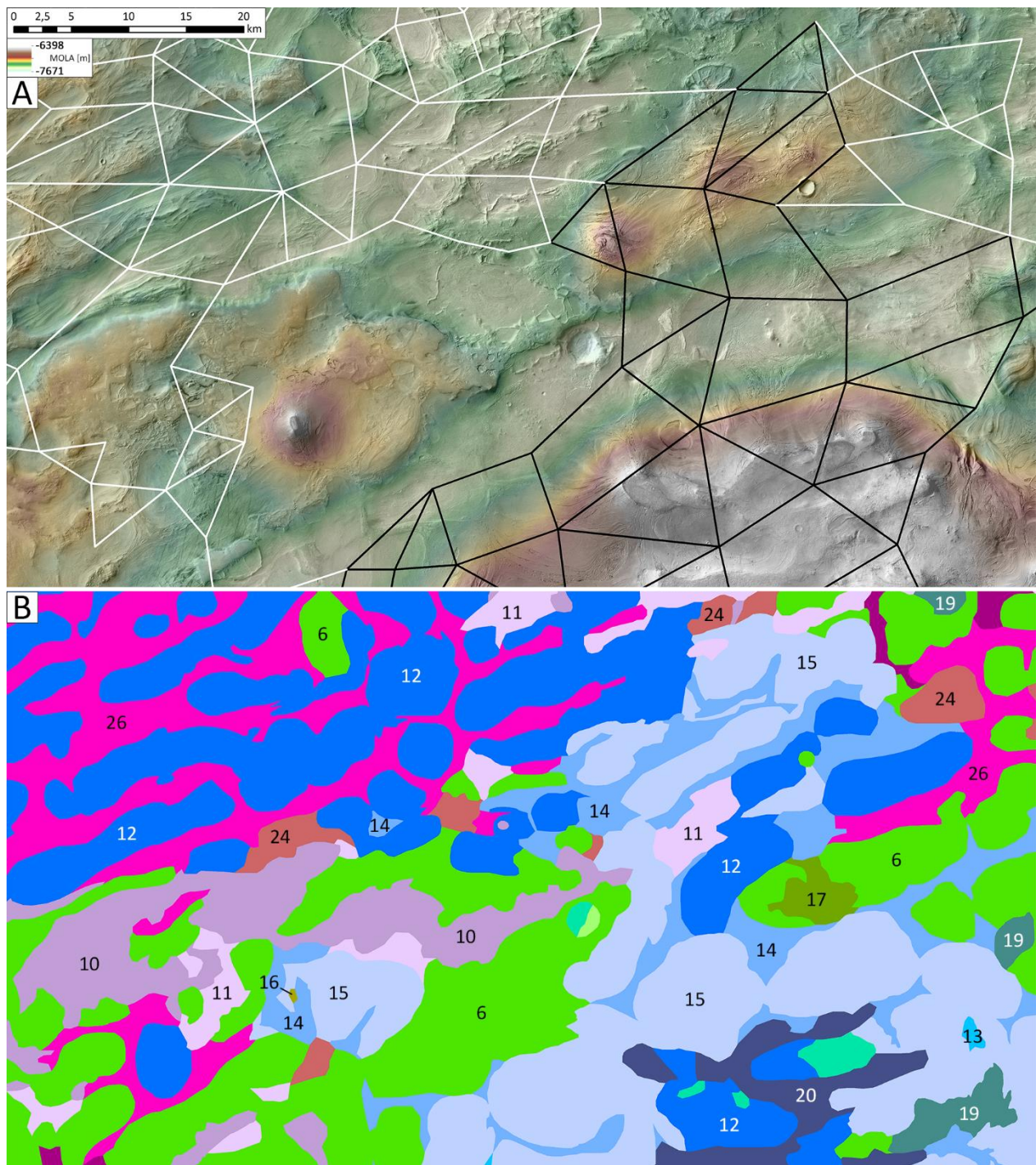
Figure 11: A) MOLA DTM superposing crop of our CTX mosaic; location shown in Fig. 1B ; north is up. The scene is centered on the southern edge of the honeycomb terrain; a portion of the elevated interior formation can be seen in the lower right. The white lines connect the centers of adjacent honeycombs (here defined as kidney/cell-like depression confined by unit HC rim ). The black lines
