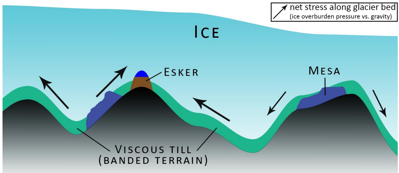
Figure 14: Illustration of our subglacial formation model for the banded terrain (see section 6.4 ).
