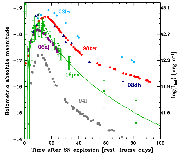
Figure 6. Pseudobolometric light curve (3000–10 000 Å) of SN 16jca after the subtraction of the host galaxy and afterglow components, compared with bolometric light curves of previous GRB-SNe 1998bw, 2003dh, 2003lw, and X-ray flash SN 2006aj (Galama et al. 1998; Malesani et al. 2004; Deng et al. 2005; Pian et al. 2006), and the ‘normal’ Type Ic SN 1994I (not associated with a GRB) (Richmond et al. 1996). Note the similarity with the light curve of SN 2006aj. To avoid confusion, the error bars are shown only for SN 16jca. The uncertainties of SN 1998bw are smaller than the markers, SN 2006aj are \sim 10 per cent, and SN 2003dh and SN 2003lw are comparable to those of SN 16jca. The first points, as in SN 2003dh, are heavily contaminated by the afterglow. The solid green line is the model light curve produced with the density and abundance structure used for the spectra modelling.
