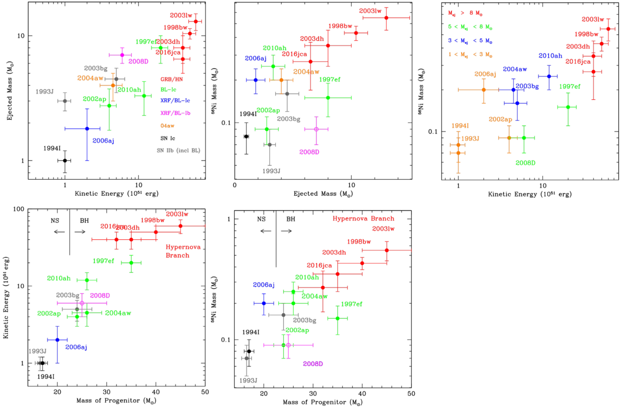
Figure 13. The location of SN 2016jca in terms of the stripped-envelope-SN correlations from Mazzali et al. (2017). For the left and middle panels, the red points are GRB-SNe, the blue points are SNe Ic associated with X-ray flashes, the pink points are SNe Ib associated with X-ray flashes, the black points are normal SNe Ic, and the grey points are normal SNe Iib. For the right top panel the SNe are coloured based on ejecta mass.
