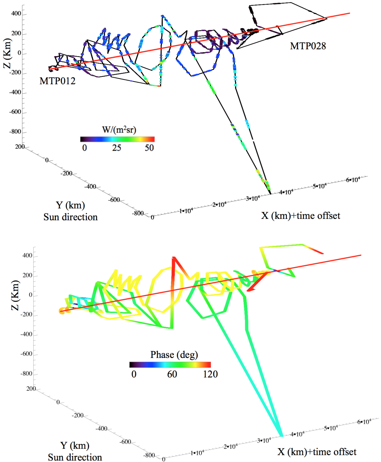
Extended Data Figure 3. Rosetta spacecraft 3d trajectory and solar phase angle variations during the time. Top panel: Rosetta trajectory in the 67P XYZ reference frame. Points along the X axis are shown starting from Rosetta's position at 2015-01-13T23:28:53 (MTP012) with an increment of 1 km every 20 minutes to improve visualization. Y axis is oriented towards the Sun and Z perpendicular to the orbital plane. The red line indicates the position of the nucleus along the X axis. The integrated radiance as measured on each
