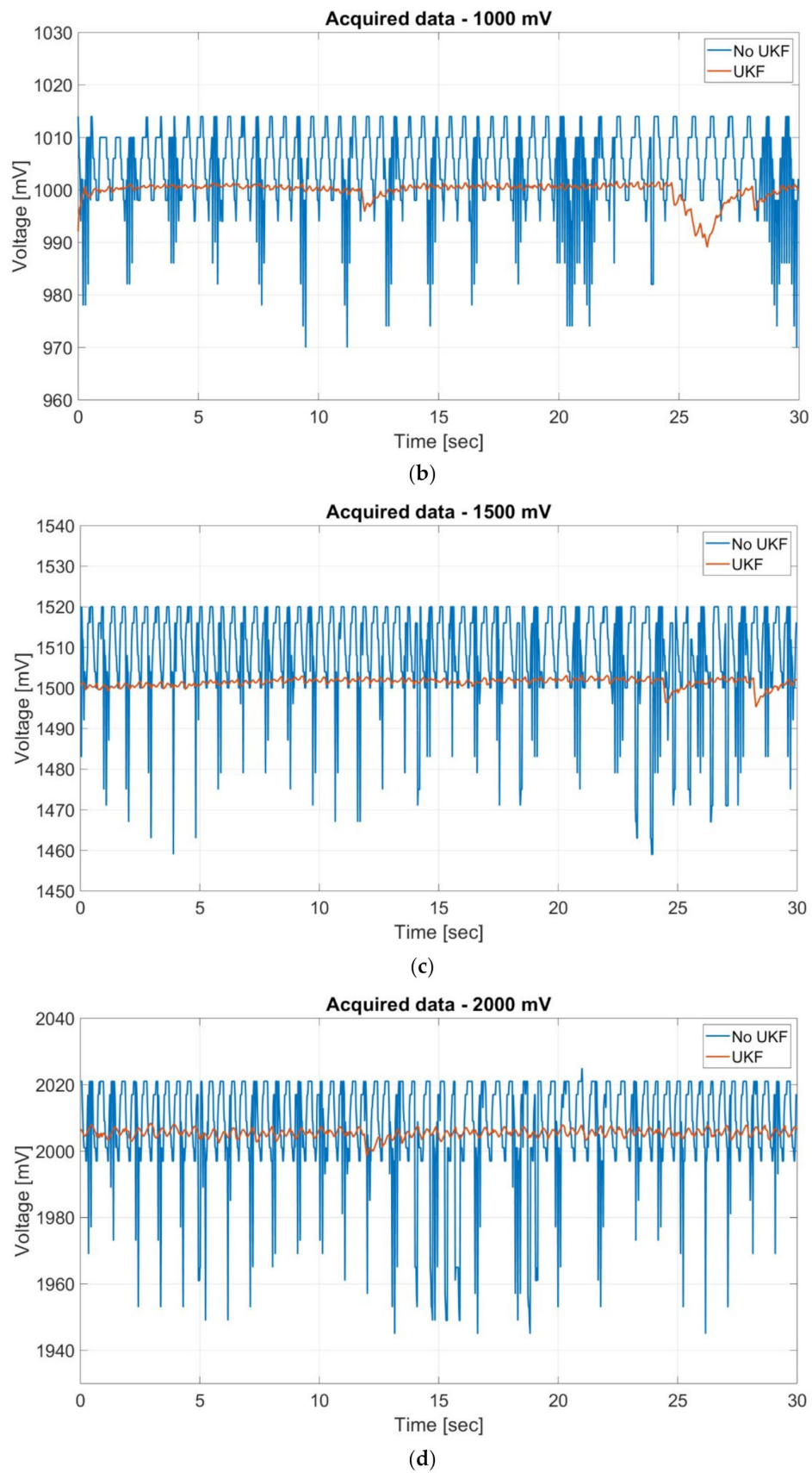
Figure 13. Graphical results of the experiment for data acquisition and elaboration: (a) acquired data at voltages of about 500 mV; (b) acquired data at voltages of about 1000 mV; (c) acquired data at voltages of about 1500 mV; (d) acquired data at voltages of about 2000 mV.
