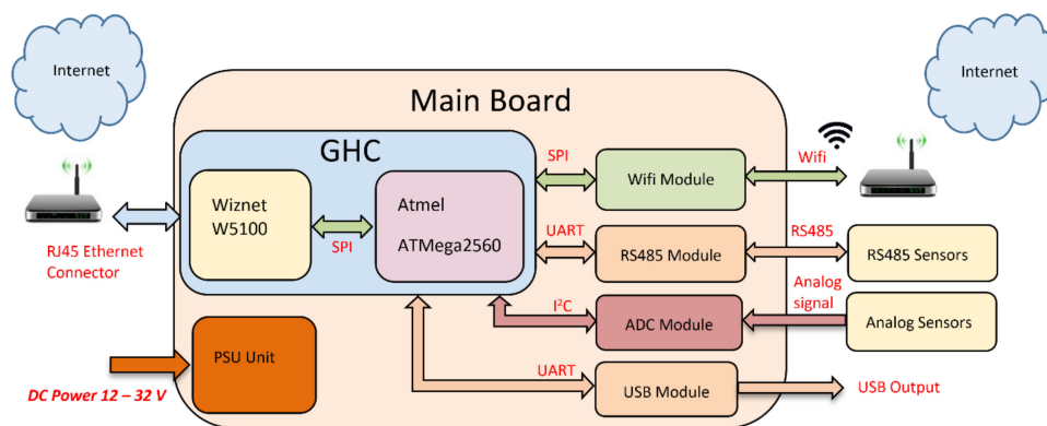
Figure 1. Block diagram of the electronic board.
