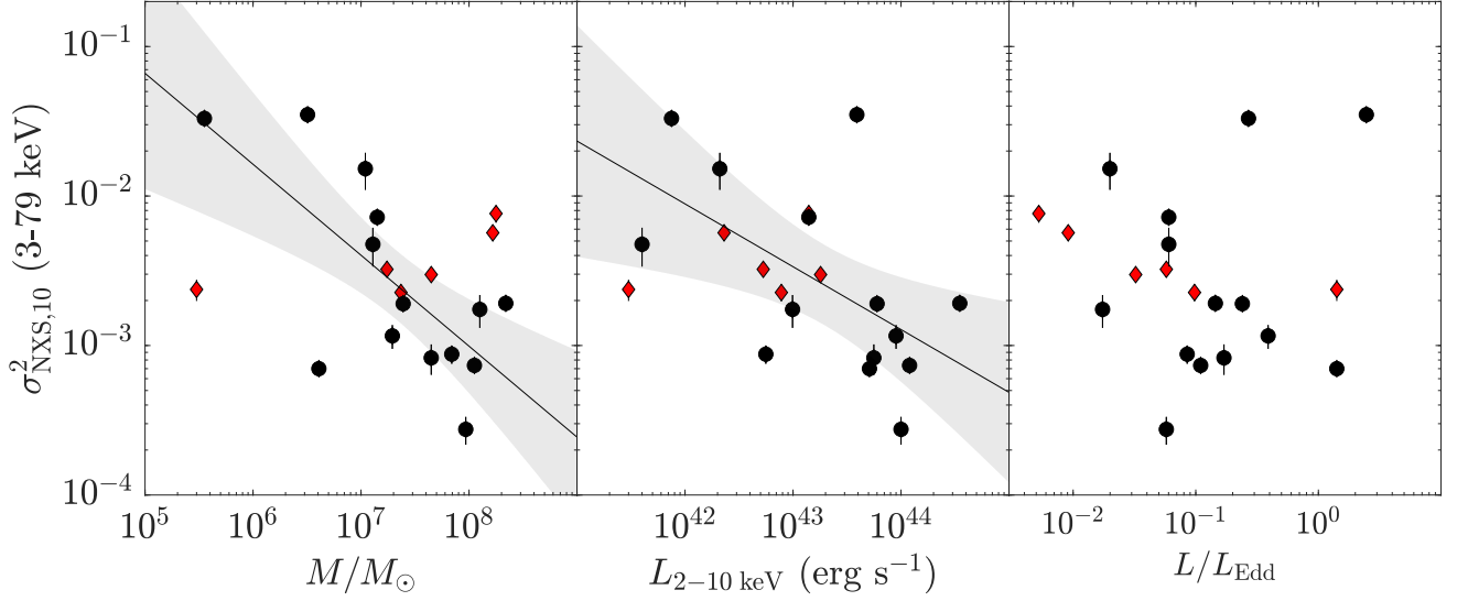
Fig. 5. Excess variance in the E = 3 - 79 keV energy band versus the black hole mass of the AGN (left). The excess variances shown here are averaged among the different epochs. A clear trend \sigma_{\text{NXS}}^2 \propto M_{\text{BH}}^{-0.6} is found with a strong anticorrelation ( r = -0.7 ). Given their large uncertainties, masses obtained with the velocity dispersion method (red diamonds) are excluded from the fit. Middle panel gives The average excess variance vs. the unabsorbed X-ray luminosity L_X is shown. We find a trend \sigma_{\text{NXS}}^2 \propto L_X^{-0.4} with moderate anticorrelation ( r = -0.5 ). Right panel shows the average excess variance vs. the Eddington ratio and no evident correlation is found. Also, in this panel, the sources with mass measurements obtained with the velocity dispersion method are drawn as red diamonds.
