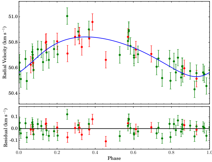
Fig. 7. Keplerian best fit to combined HET HRS and TNG HARPS-N data for BD+03 2562. The jitter is added to the uncertainties.
