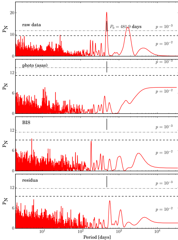
Fig. 8. Same as Fig. 6 but for BD+03 2562.
